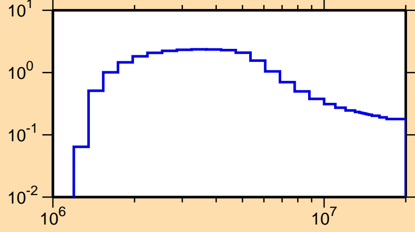
\sigma vs. E for ^{144}\text{La}(n,n\text{cont.})
