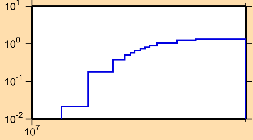
\sigma vs. E for ^{144}\text{La}(n,3n)
