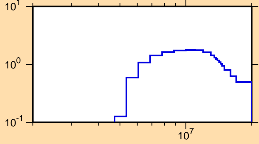
\sigma vs. E for ^{144}\text{La}(n,2n)
