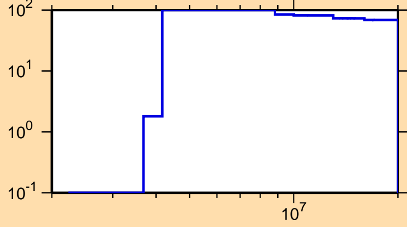
\Delta\sigma/\sigma vs. E for ^{144}\text{La}(n,p)
