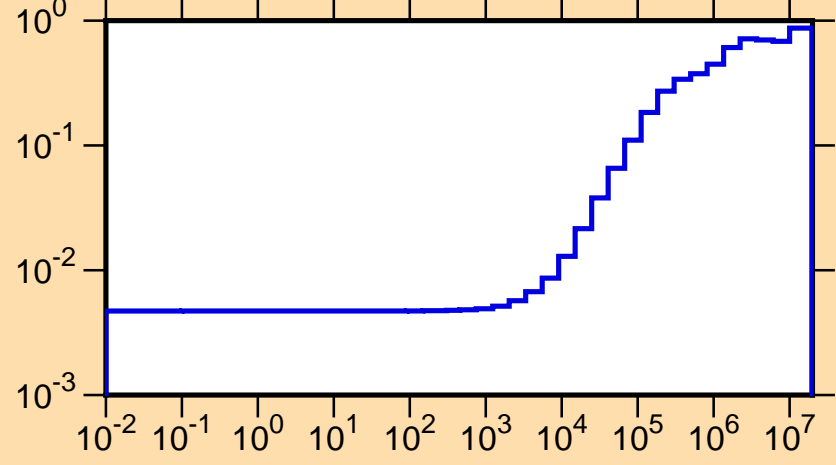
\mu vs. E for ^{144}\text{La} (mt251)
