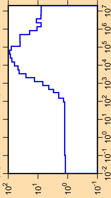
\Delta\mu/\mu vs. E for ^{144}\text{La} (mt251)
