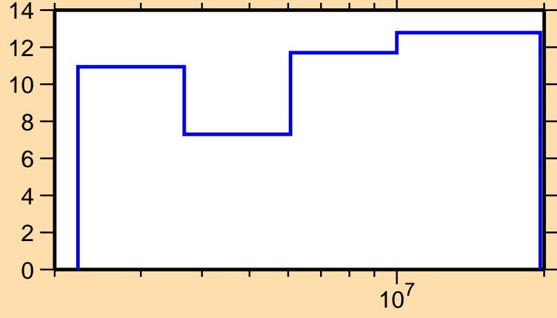
\Delta\sigma/\sigma vs. E for ^{144}\text{La}(n,n\text{cont.})
