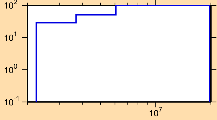
\Delta\sigma/\sigma vs. E for ^{144}\text{La}(n,n_1)
