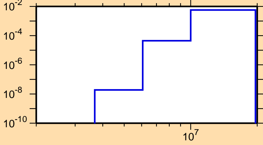
\sigma vs. E for ^{144}\text{La}(n,p)
