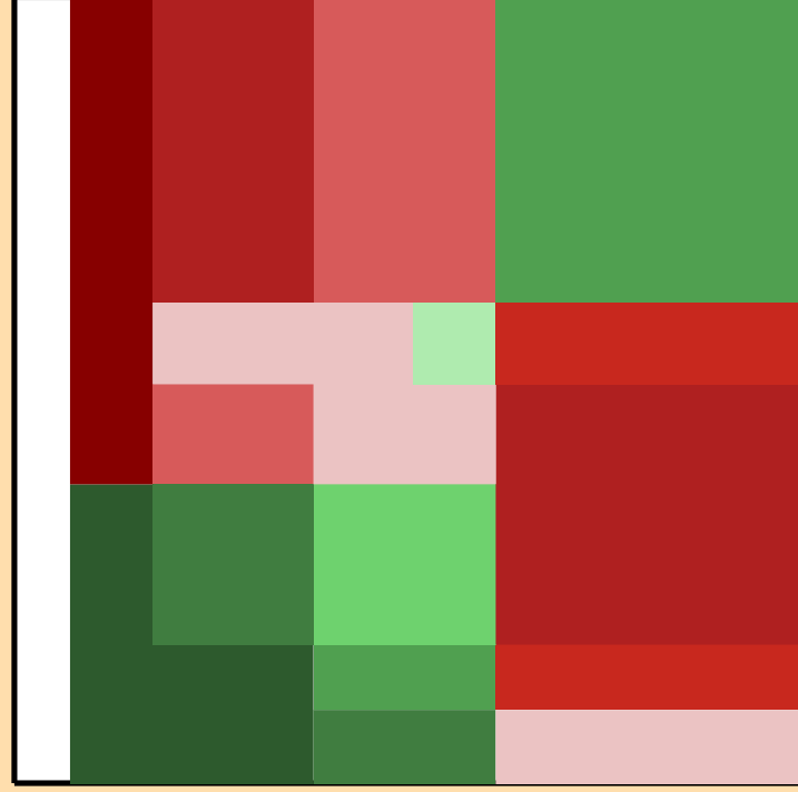
\Delta\sigma/\sigma vs. E for ^{144}\text{La}(n,p)
