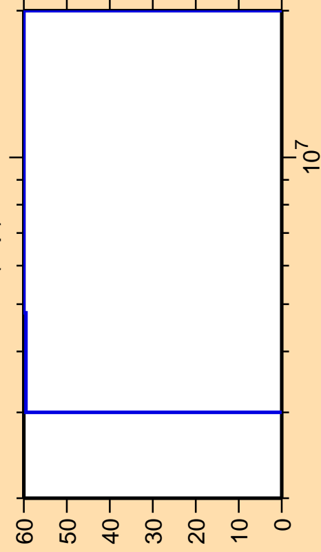
\Delta\sigma/\sigma vs. E for ^{144}\text{La}(n,p)
