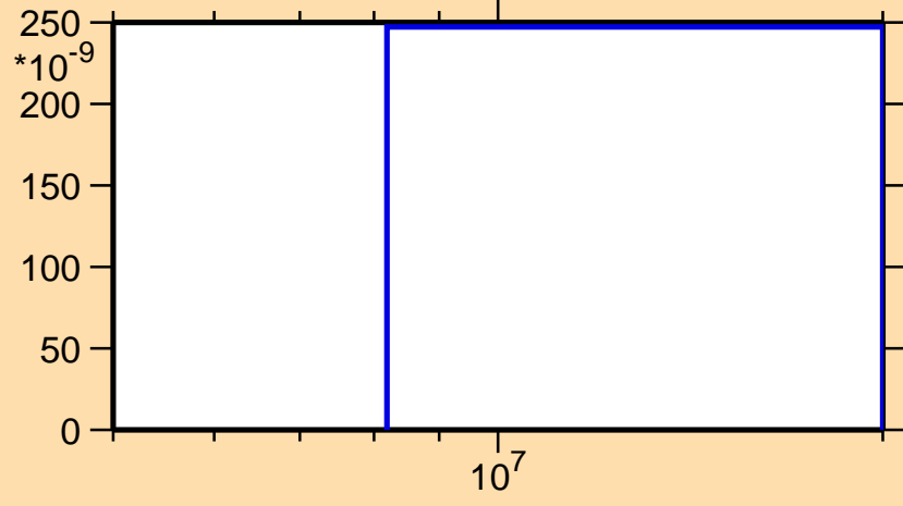
\sigma vs. E for ^{144}\text{La}(n,2n\alpha)
