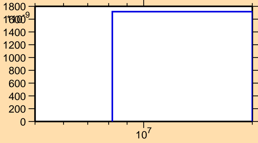
\sigma vs. E for ^{144}\text{La}(n,nt)
