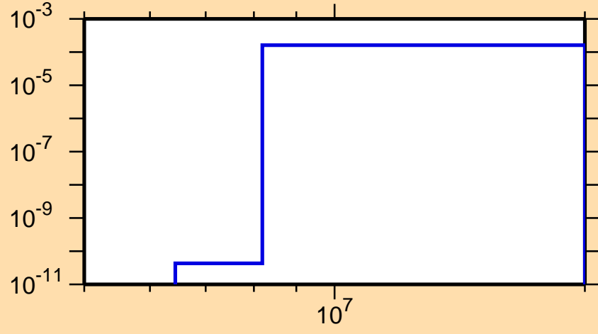
\sigma vs. E for ^{144}\text{La}(n,t)
