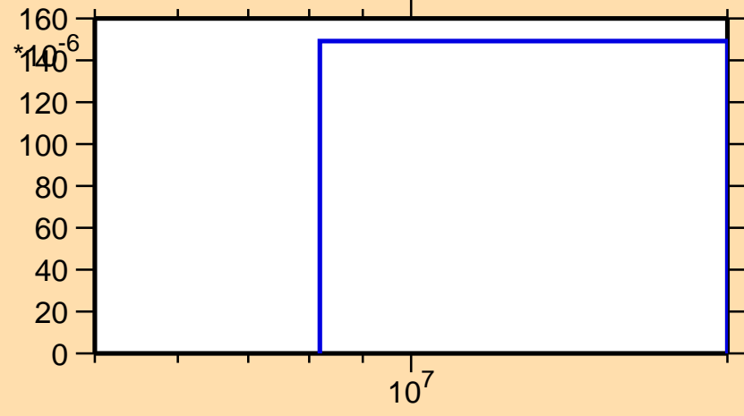
\sigma vs. E for ^{144}\text{La}(n,np)
