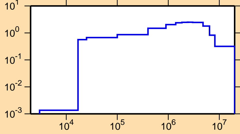
\sigma vs. E for ^{144}\text{La}(n,\text{inel.})
