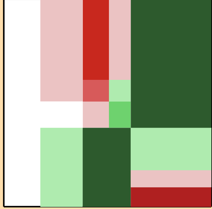
\Delta\sigma/\sigma vs. E for ^{144}\text{La}(n,2n)
