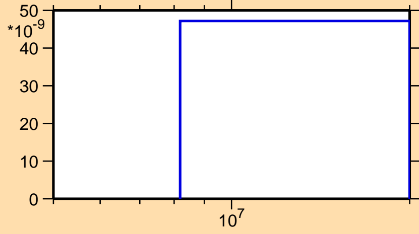
\sigma vs. E for ^{144}\text{La}(n,2np)
