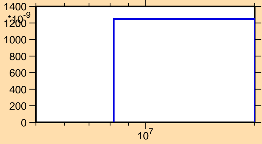
\sigma vs. E for ^{144}\text{La}(n,\text{nd})
