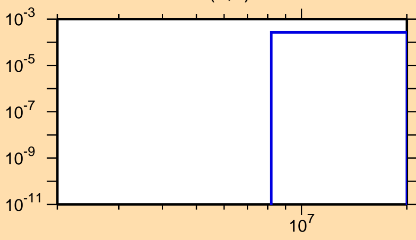
\sigma vs. E for ^{144}\text{La}(n,d)
