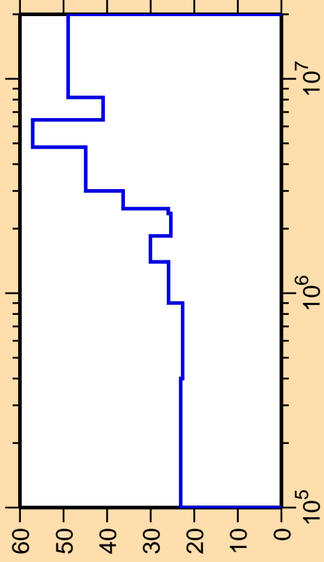
\Delta\sigma/\sigma vs. E for ^{144}\text{La}(n,n_4)
