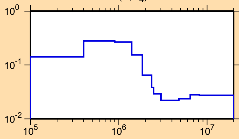
\sigma vs. E for ^{144}\text{La}(n,n_4)
