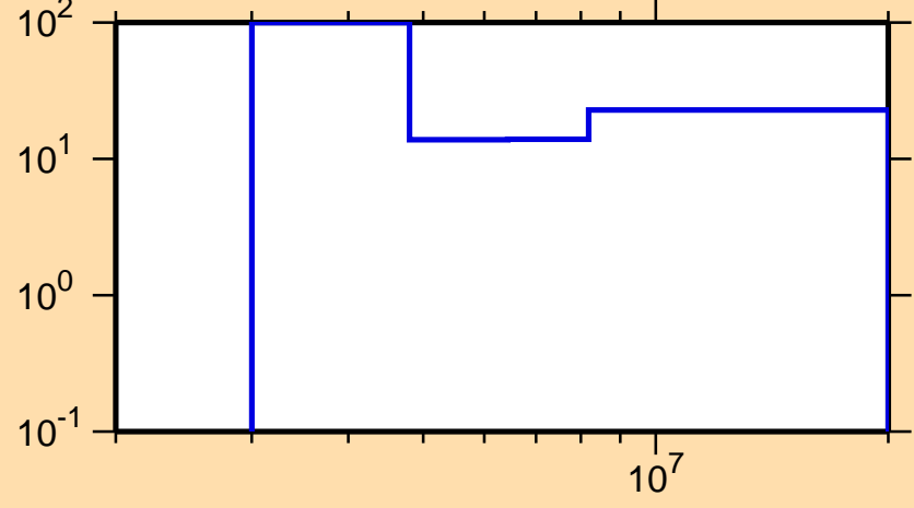
\Delta\sigma/\sigma vs. E for ^{144}\text{La}(n,2n)
