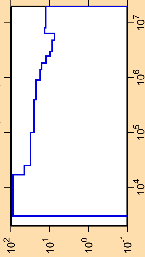
\Delta\sigma/\sigma vs. E for ^{144}\text{La}(n,\text{inel.})
