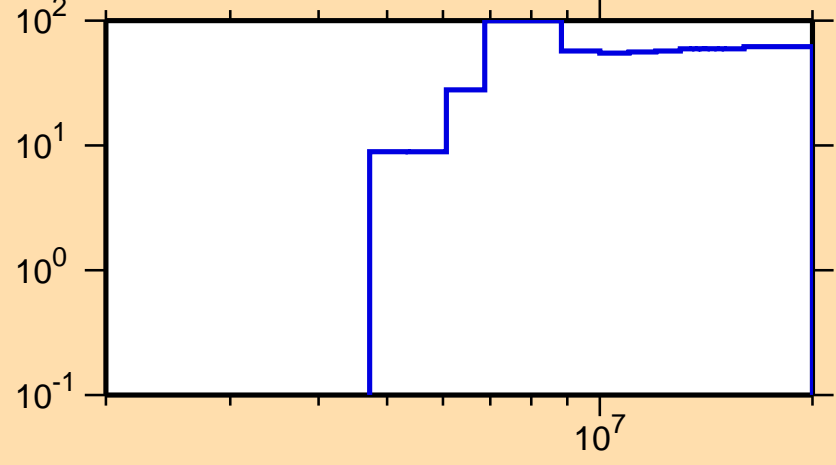
\Delta\sigma/\sigma vs. E for ^{145}\text{La}(n,ncont.)
