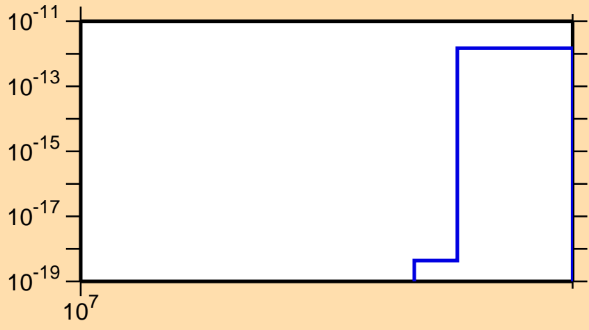
\sigma vs. E for ^{145}\text{La} (mt 11)
