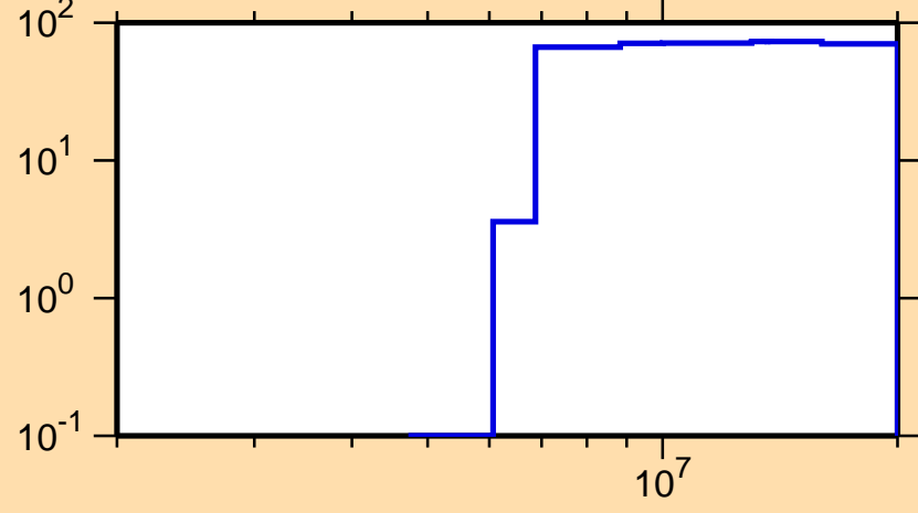
\Delta\sigma/\sigma vs. E for ^{145}\text{La}(n,p)
