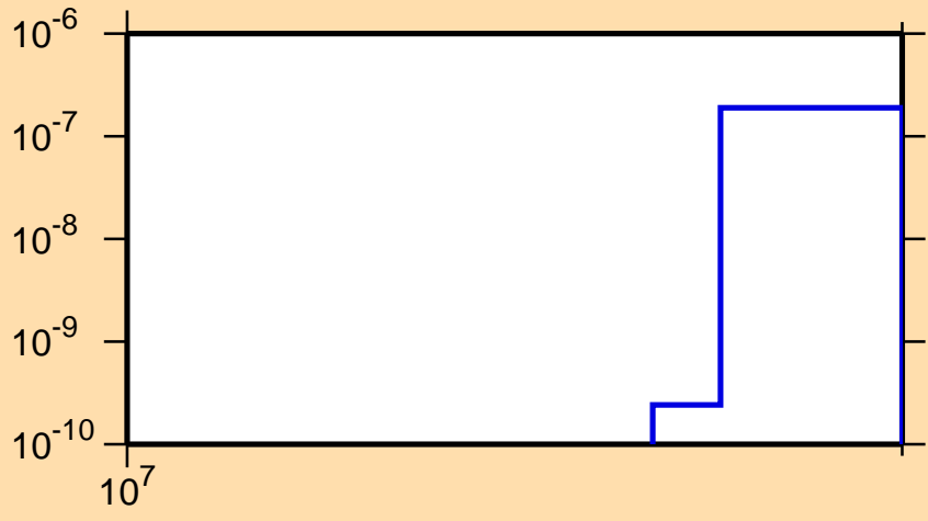
\sigma vs. E for ^{145}\text{La}(n,2np)
