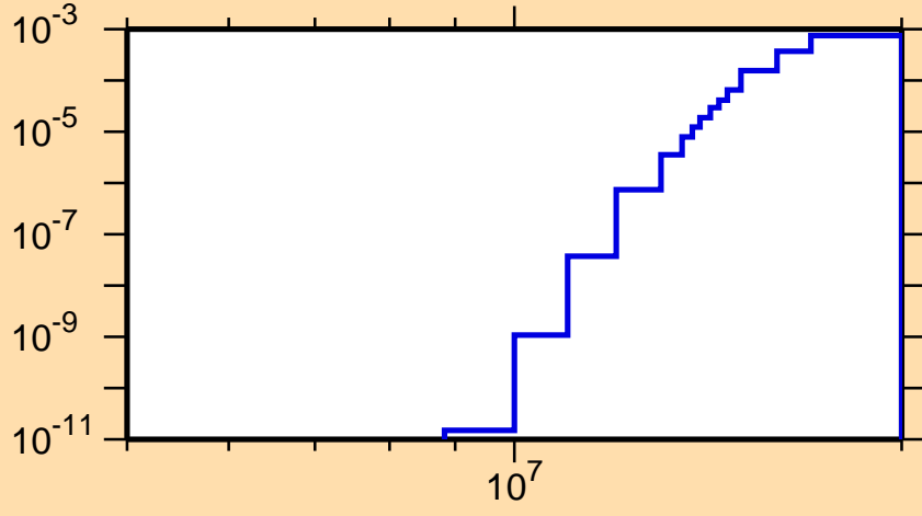
\sigma vs. E for ^{145}\text{La}(n,t)
