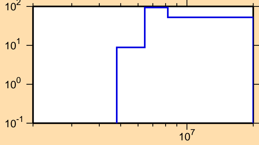
\Delta\sigma/\sigma vs. E for ^{145}\text{La}(n,n\text{cont.})
