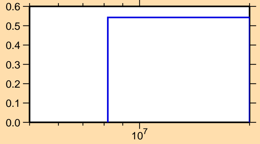
\sigma vs. E for ^{145}\text{La}(n,3n)
