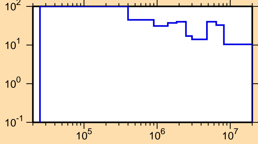
\Delta\sigma/\sigma vs. E for ^{145}\text{La}(n,\text{el.})
