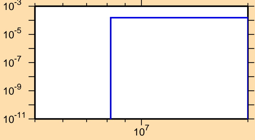
\sigma vs. E for ^{145}\text{La}(n,d)
