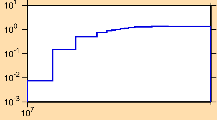
\sigma vs. E for ^{146}\text{La}(n,3n)
