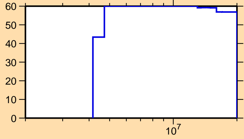
\Delta\sigma/\sigma vs. E for ^{146}\text{La}(n,ncont.)
