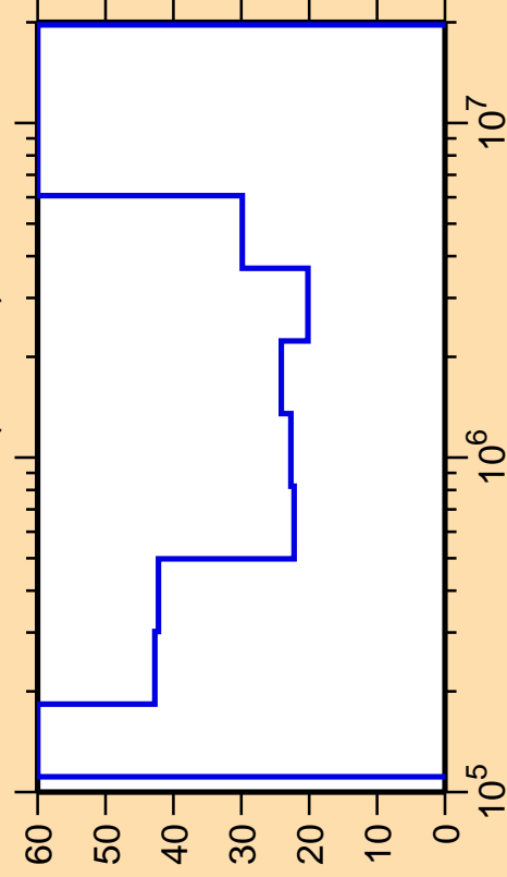
\Delta\sigma/\sigma vs. E for ^{146}\text{La}(n,\text{inel.})
