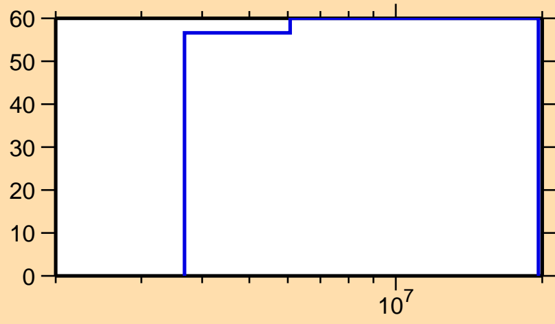
\Delta\sigma/\sigma vs. E for ^{146}\text{La}(n,p)
