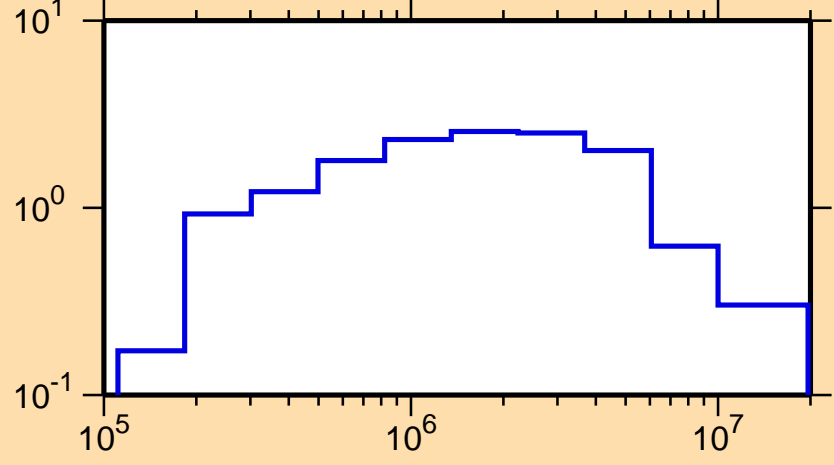
\sigma vs. E for ^{146}\text{La}(n,\text{inel.})
