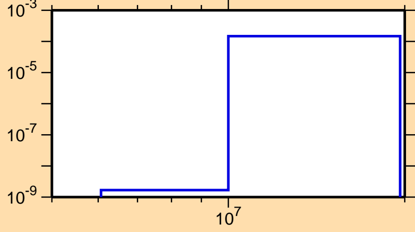
\sigma vs. E for ^{146}\text{La}(n,t)
