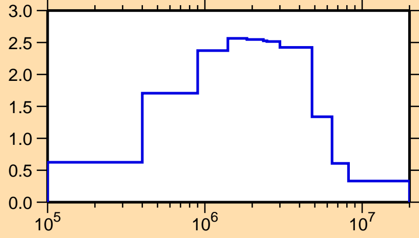
\sigma vs. E for ^{146}\text{La}(n,\text{inel.})
