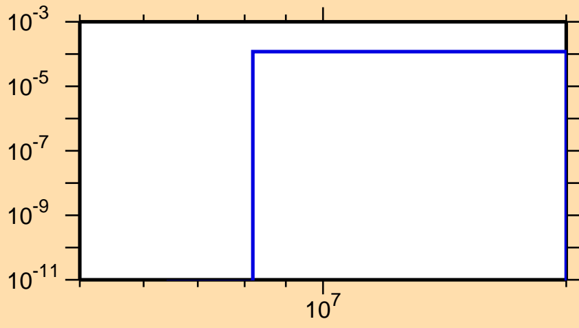
\sigma vs. E for ^{146}\text{La}(n,t)
