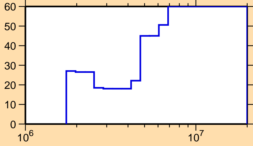
\Delta\sigma/\sigma vs. E for ^{146}\text{La}(n,n\text{cont.})
