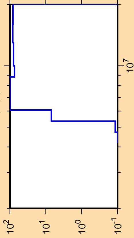
\Delta\sigma/\sigma vs. E for ^{146}\text{La}(n,p)
