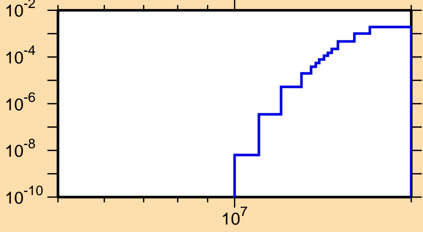
\sigma vs. E for ^{146}\text{La}(n,d)
