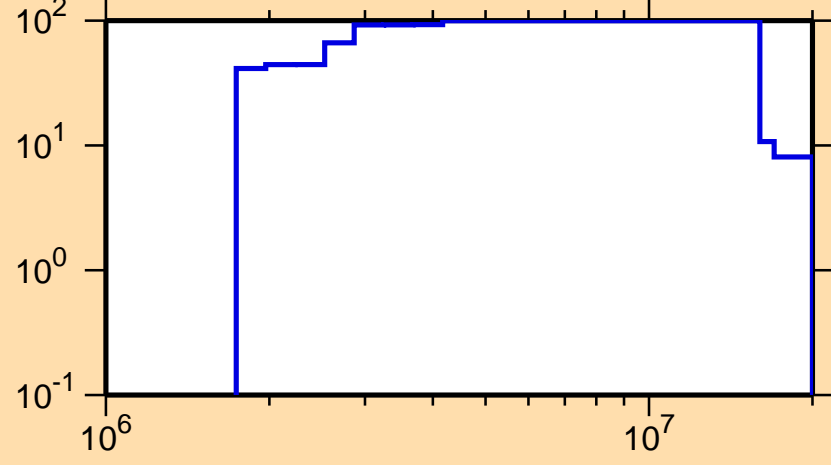
\Delta\sigma/\sigma vs. E for ^{146}\text{La}(n,n_1)
