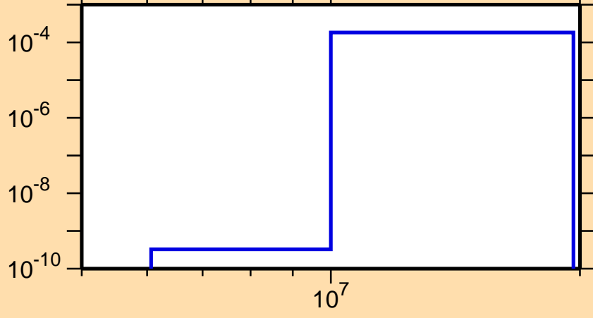
\sigma vs. E for ^{146}\text{La}(n,t)
