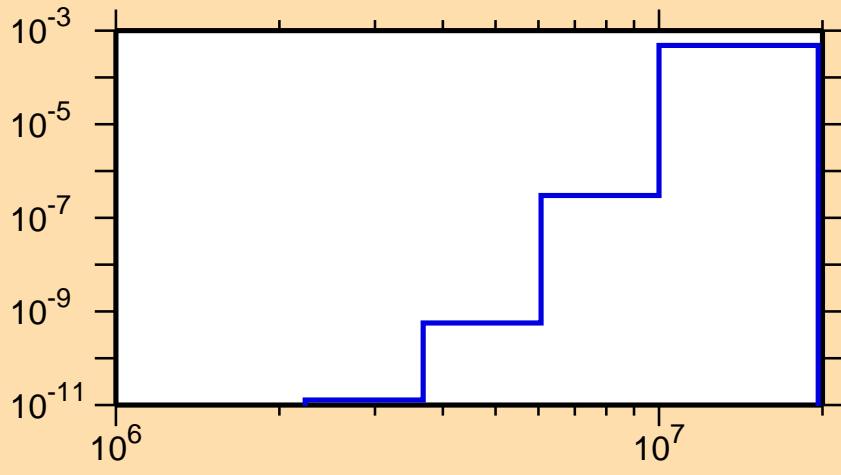
\sigma vs. E for ^{146}\text{La}(n,\alpha)
