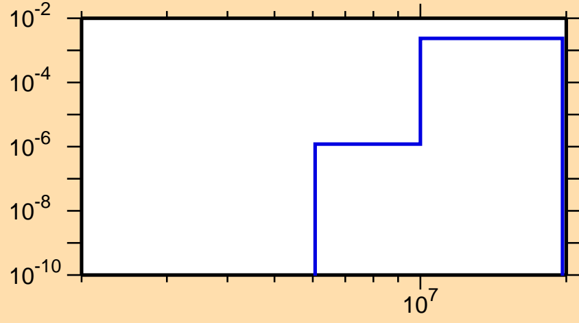
\sigma vs. E for ^{146}\text{La}(n,p)
