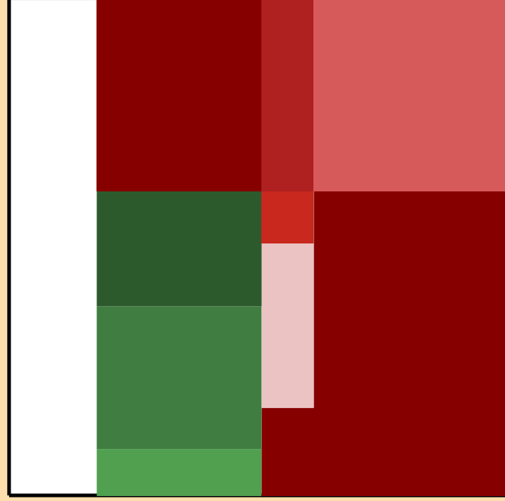
\Delta\sigma/\sigma vs. E for ^{146}\text{La}(n,p)
