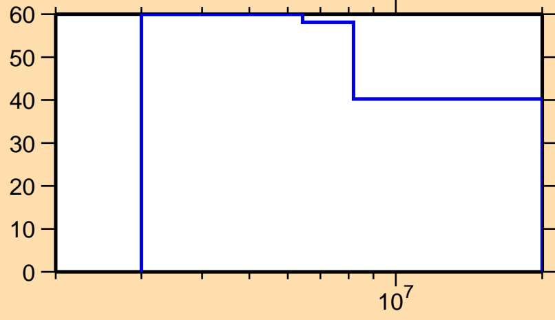
\Delta\sigma/\sigma vs. E for ^{146}\text{La}(n,el.)
