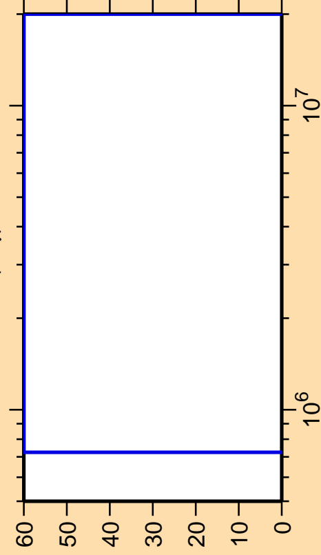
\Delta\sigma/\sigma vs. E for ^{147}\text{La}(n,\gamma)
