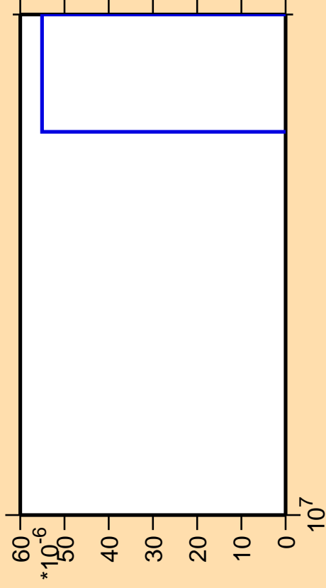
\Delta\sigma/\sigma vs. E for ^{147}\text{La} (mt 42)
