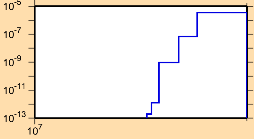
\sigma vs. E for ^{147}\text{La}(n,\text{nd})
