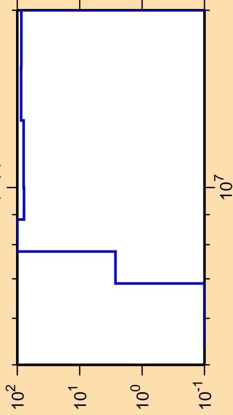
\Delta\sigma/\sigma vs. E for ^{147}\text{La}(n,p)
