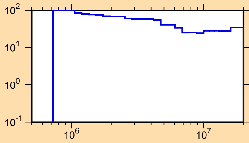
\Delta\sigma/\sigma vs. E for ^{147}\text{La}(n,n\text{cont.})
