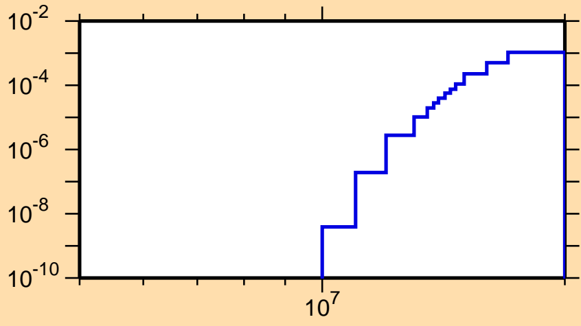
\sigma vs. E for ^{147}\text{La}(n,d)
