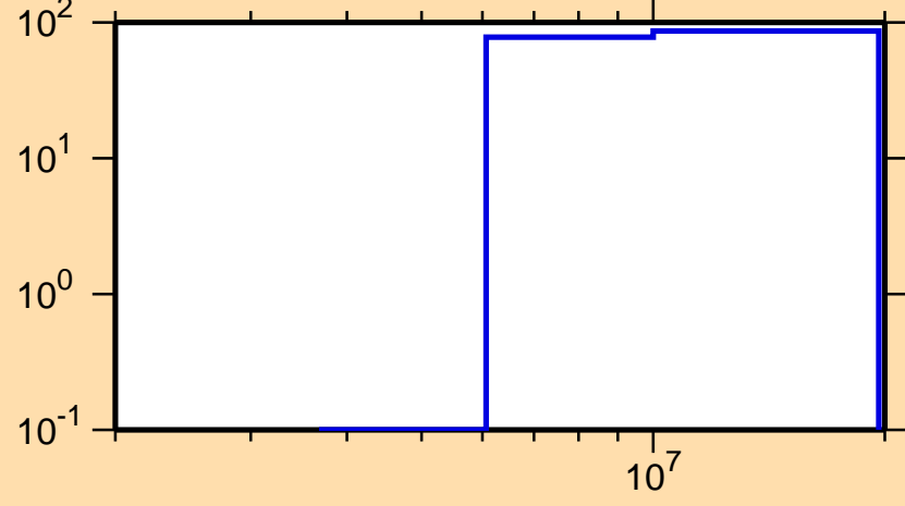
\Delta\sigma/\sigma vs. E for ^{147}\text{La}(n,p)
