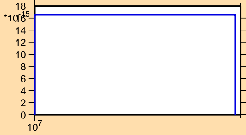
\sigma vs. E for ^{147}\text{La}(n,3n\alpha)
