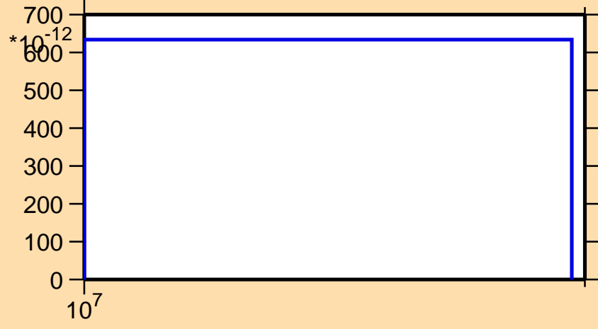
\sigma vs. E for ^{147}\text{La}(n,2np)
