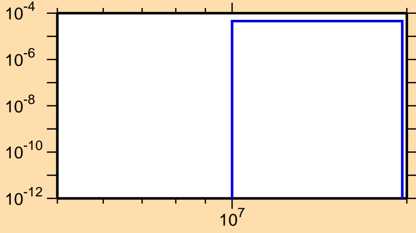
\sigma vs. E for ^{147}\text{La}(n,t)
