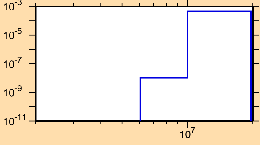
\sigma vs. E for ^{147}\text{La}(n,p)
