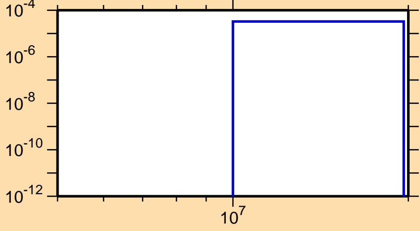
\sigma vs. E for ^{147}\text{La}(n,np)
