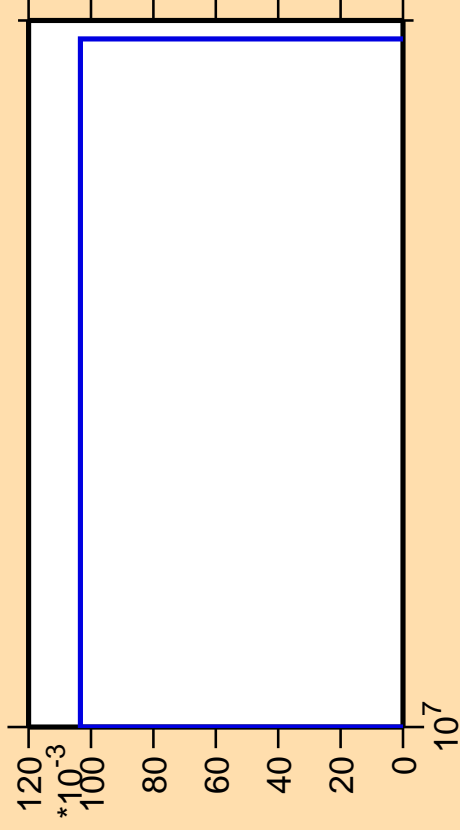
\Delta\sigma/\sigma vs. E for ^{147}\text{La} (mt 11)
