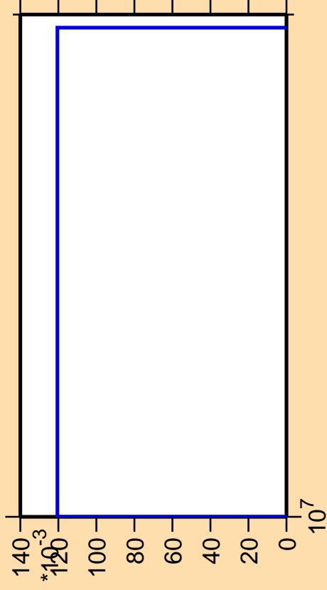
\Delta\sigma/\sigma vs. E for ^{147}\text{La}(n,3n\alpha)
