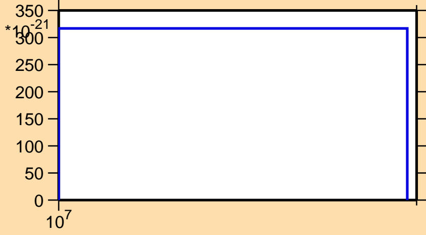
\sigma vs. E for ^{147}\text{La} (mt 42)
