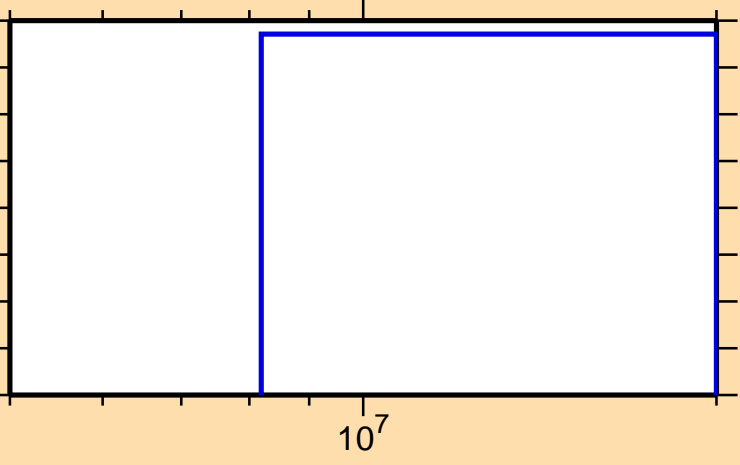
\sigma vs. E for ^{147}\text{La}(n,d)
