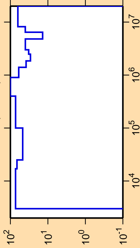
\Delta\sigma/\sigma vs. E for ^{147}\text{La}(n,\text{inel.})
