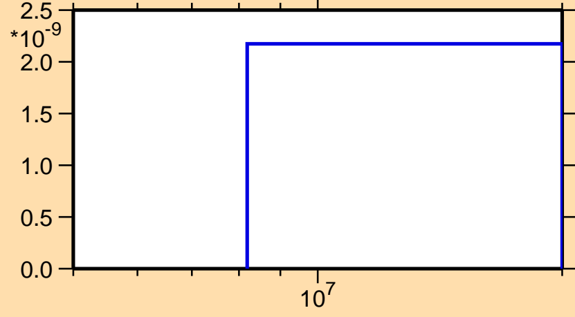
\sigma vs. E for ^{147}\text{La}(n,2n\alpha)
