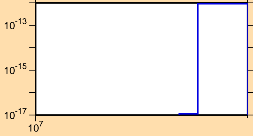
\sigma vs. E for ^{148}\text{La}(n,3n\alpha)
