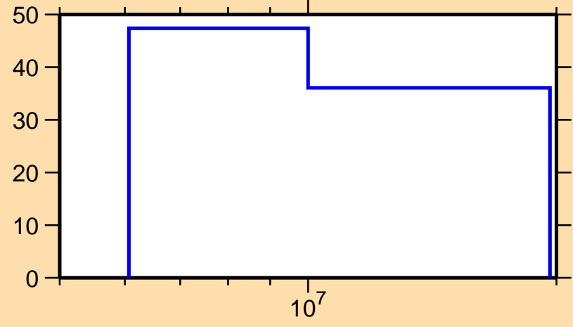
\Delta\sigma/\sigma vs. E for ^{148}\text{La}(n,n\text{cont.})
