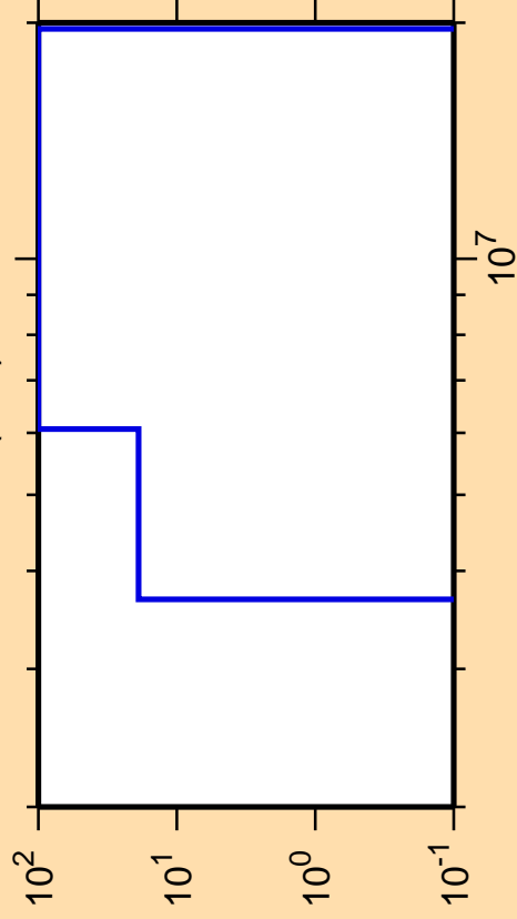
\Delta\sigma/\sigma vs. E for ^{148}\text{La}(n,\alpha)
