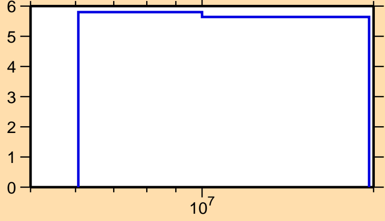
\Delta\sigma/\sigma vs. E for ^{148}\text{La}(n,\text{tot.})
