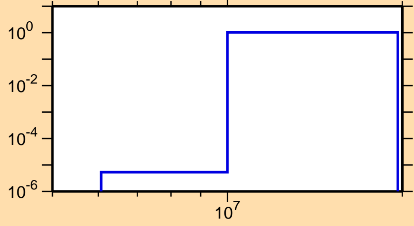
\sigma vs. E for ^{148}\text{La}(n,3n)
