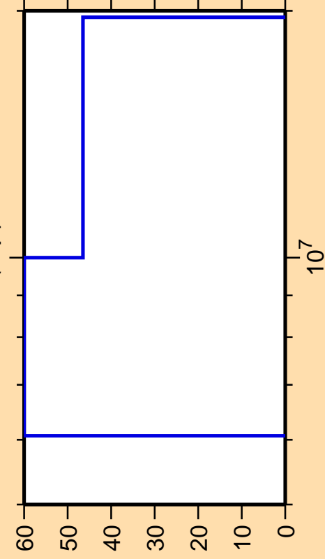
\Delta\sigma/\sigma vs. E for ^{148}\text{La}(n,p)
