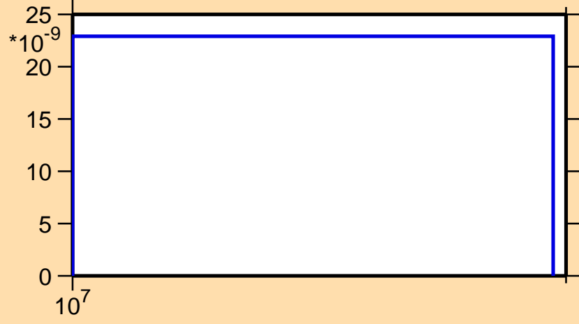
\sigma vs. E for ^{148}\text{La}(n,2n\alpha)
