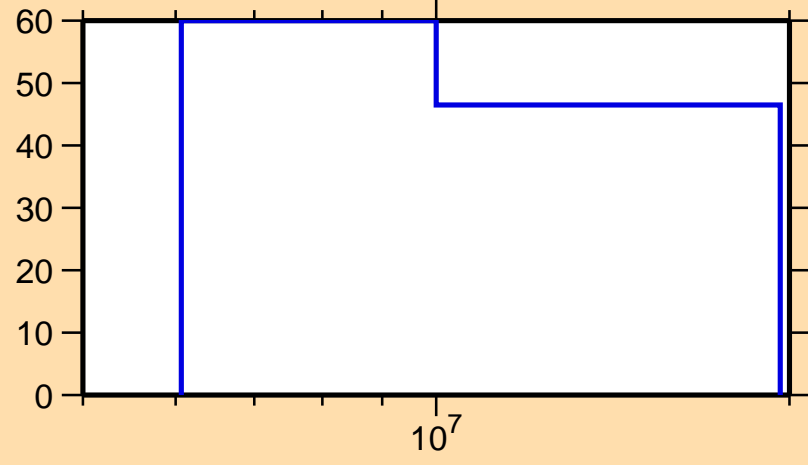
\Delta\sigma/\sigma vs. E for ^{148}\text{La}(n,p)
