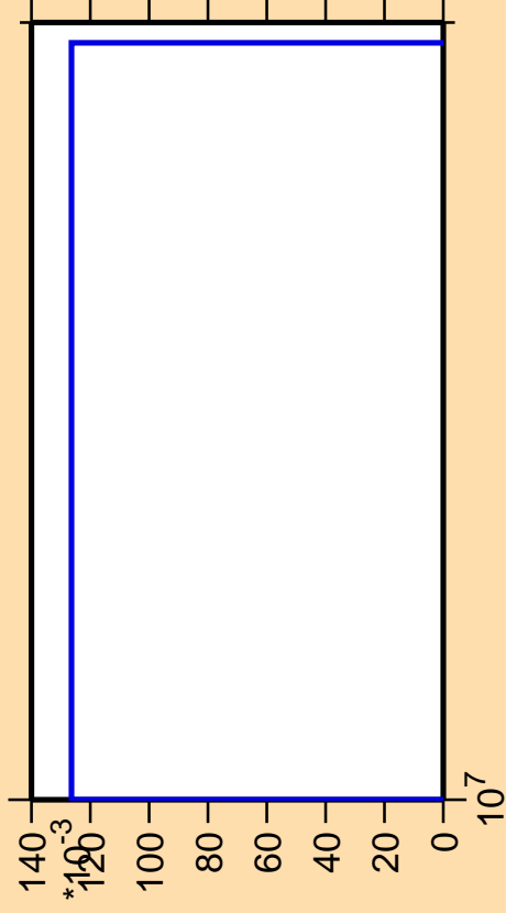
\Delta\sigma/\sigma vs. E for ^{148}\text{La} (mt 11)
