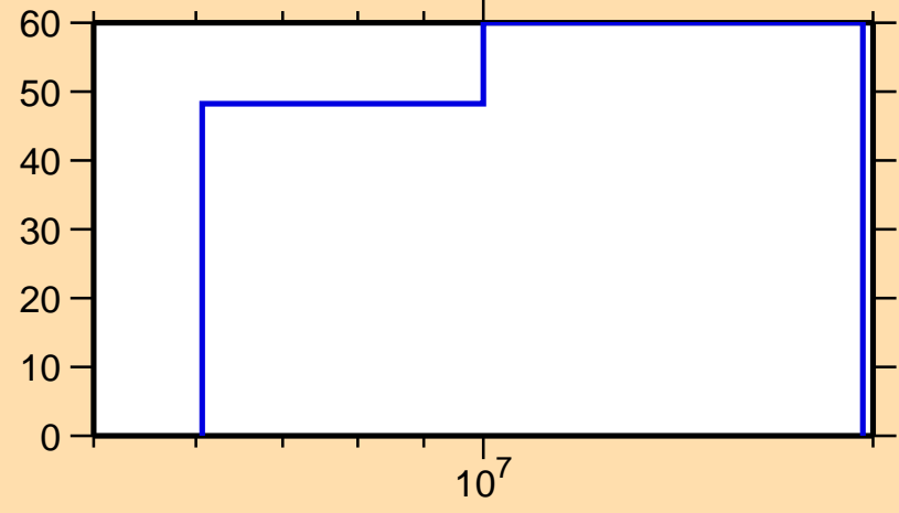
\Delta\sigma/\sigma vs. E for ^{148}\text{La}(n,\gamma)
