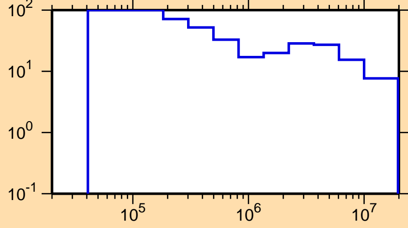
\Delta\sigma/\sigma vs. E for ^{148}\text{La}(n,\text{el.})
