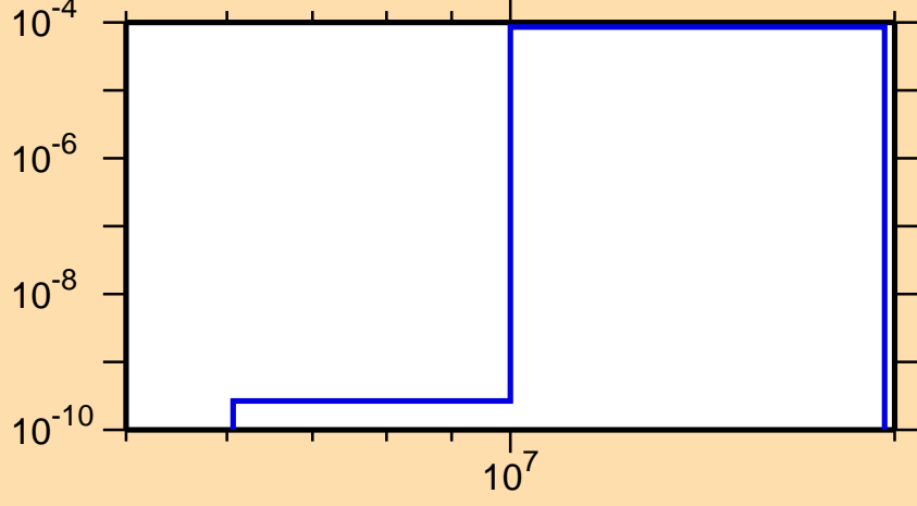
\sigma vs. E for ^{148}\text{La}(n,t)
