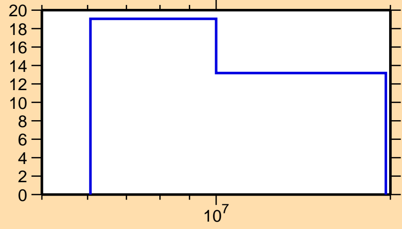
\Delta\sigma/\sigma vs. E for ^{148}\text{La}(n,2n)
