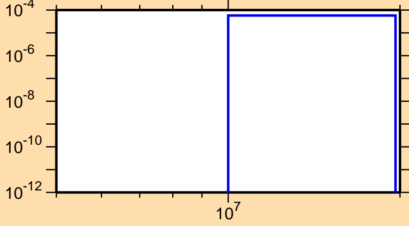
\sigma vs. E for ^{148}\text{La}(n,d)
