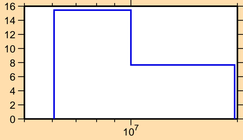
\Delta\sigma/\sigma vs. E for ^{148}\text{La}(n,el.)
