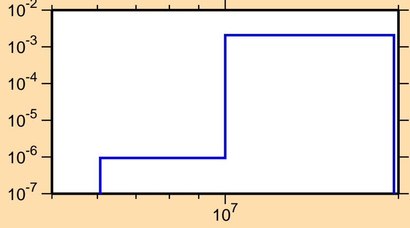
\sigma vs. E for ^{148}\text{La}(n,p)
