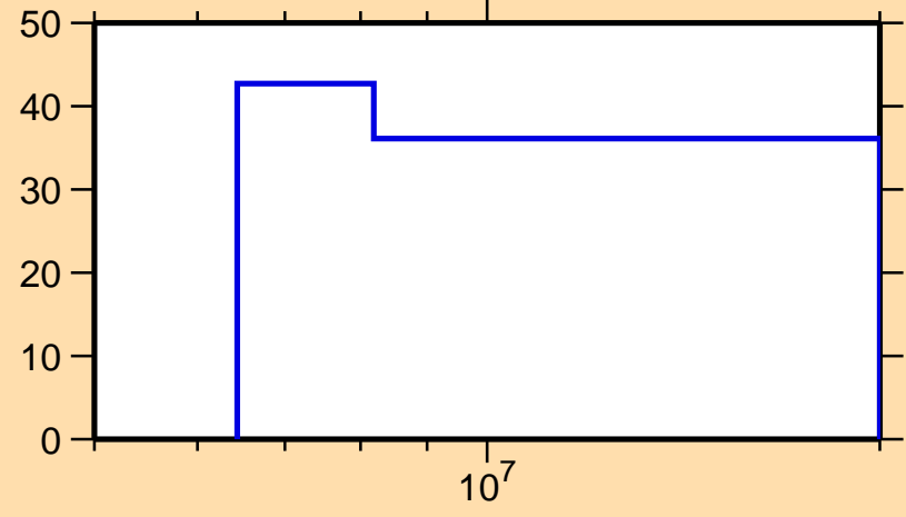
\Delta\sigma/\sigma vs. E for ^{148}\text{La}(n,ncont.)
