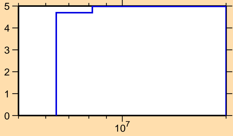
\Delta\sigma/\sigma vs. E for ^{148}\text{La}(n,\text{tot.})
