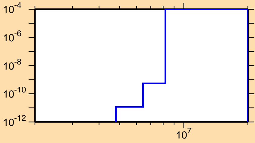
\sigma vs. E for ^{148}\text{La}(n,\alpha)
