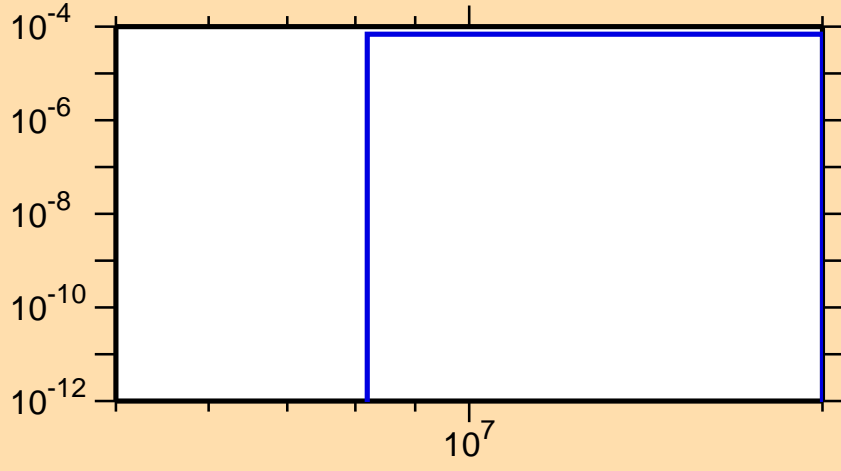
\sigma vs. E for ^{148}\text{La}(n,t)
