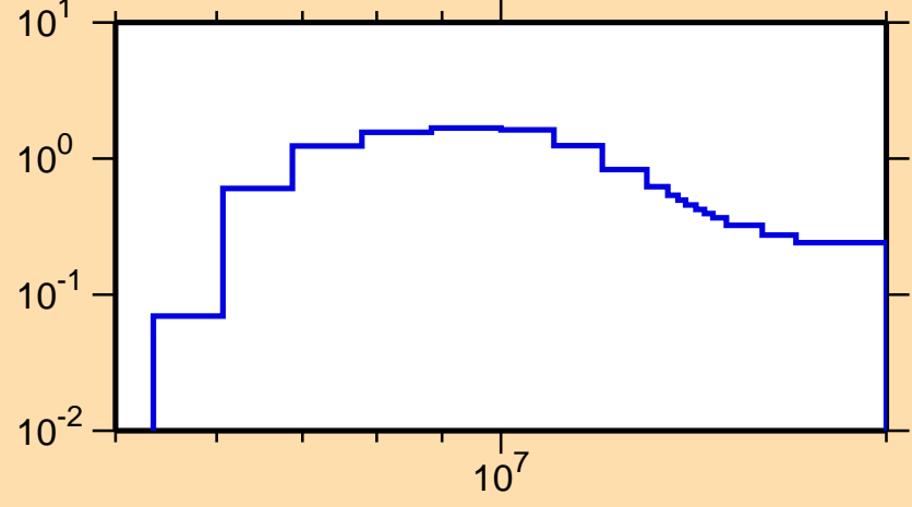
\sigma vs. E for ^{149}\text{La}(n,2n)
