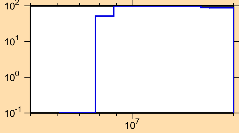
\Delta\sigma/\sigma vs. E for ^{149}\text{La}(n,p)
