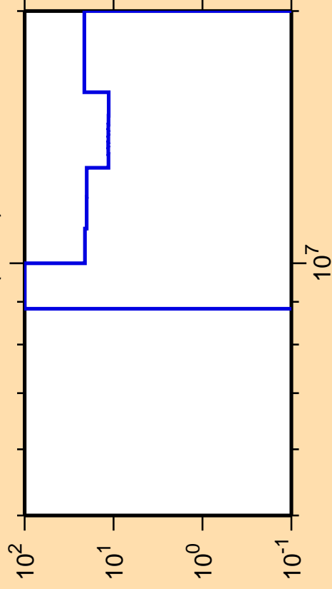
\Delta\sigma/\sigma vs. E for ^{149}\text{La}(n,3n)
