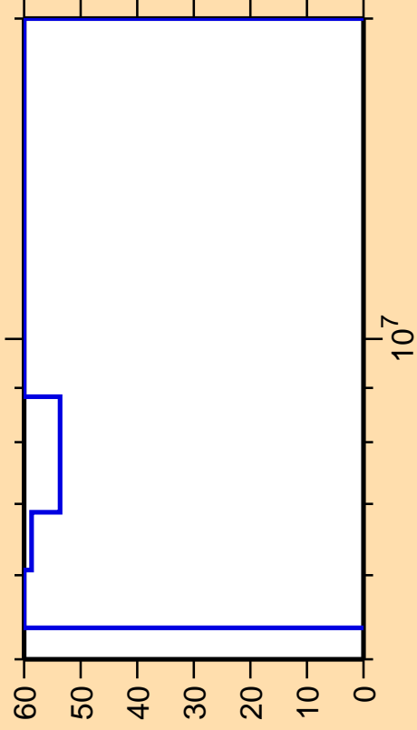
\Delta\sigma/\sigma vs. E for ^{149}\text{La}(n,n_1)
