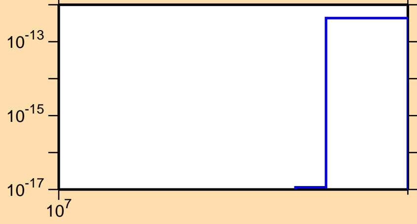
\sigma vs. E for ^{149}\text{La}(n,3n\alpha)
