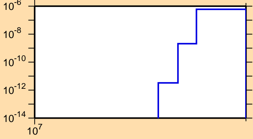
\sigma vs. E for ^{149}\text{La}(n,\text{nd})
