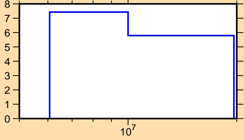
\Delta\sigma/\sigma vs. E for ^{149}\text{La}(n,\text{tot.})
