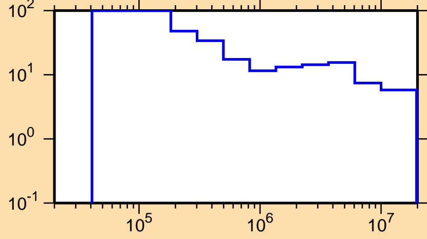
\Delta\sigma/\sigma vs. E for ^{149}\text{La}(n,\text{tot.})
