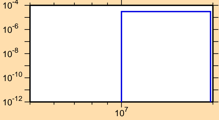
\sigma vs. E for ^{149}\text{La}(n,d)
