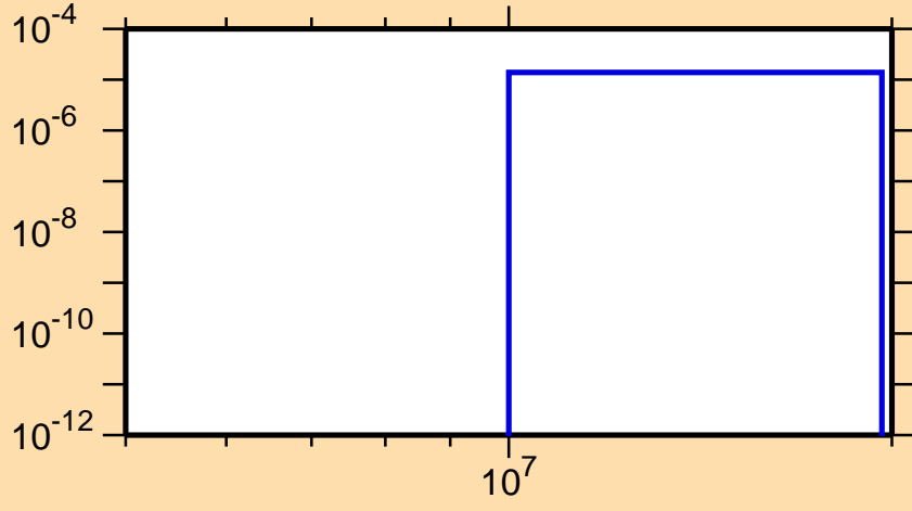
\sigma vs. E for ^{149}\text{La}(n,t)
