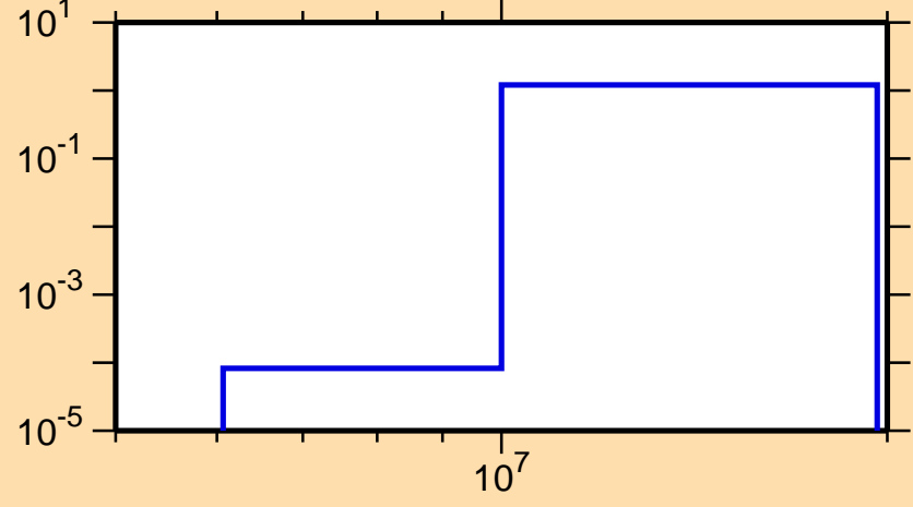
\sigma vs. E for ^{149}\text{La}(n,3n)
