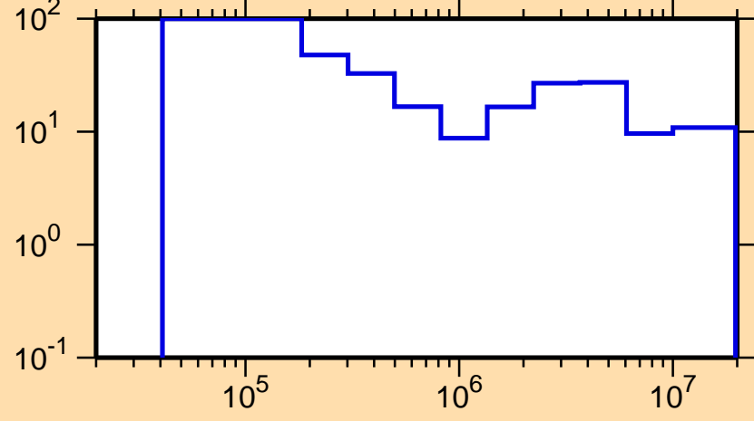
\Delta\sigma/\sigma vs. E for ^{149}\text{La}(n,\text{el.})
