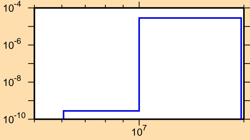
\sigma vs. E for ^{149}\text{La}(n,\alpha)
