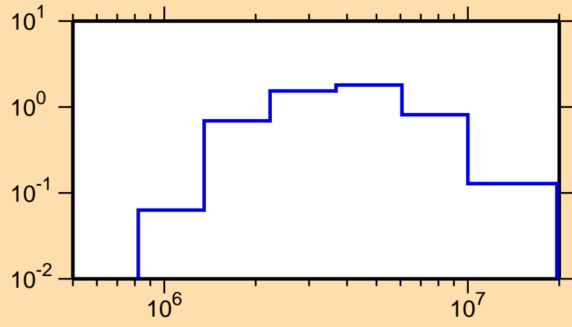
\sigma vs. E for ^{149}\text{La}(n,n\text{cont.})
