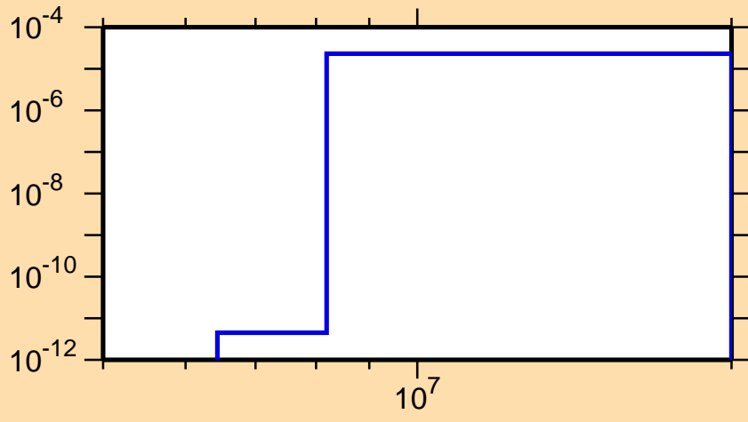
\sigma vs. E for ^{149}\text{La}(n,\alpha)
