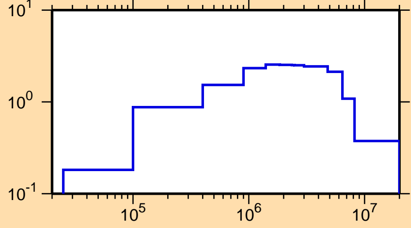
\sigma vs. E for ^{149}\text{La}(n,\text{inel.})
