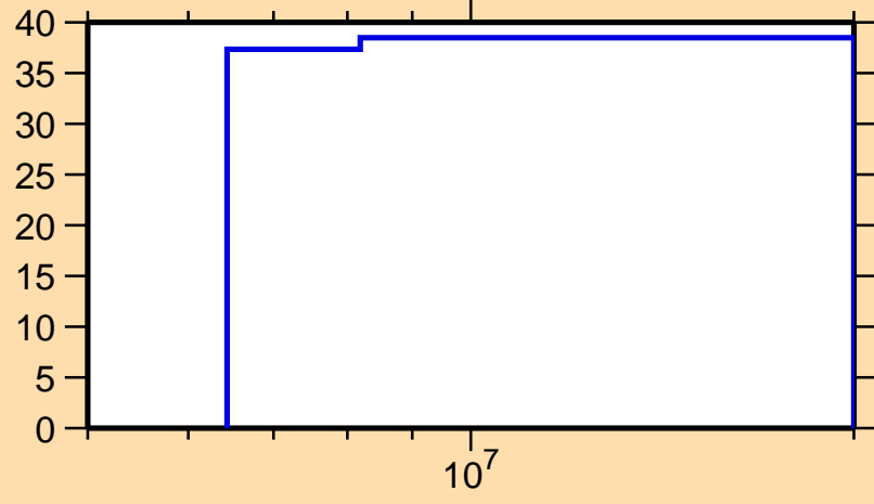
\Delta\sigma/\sigma vs. E for ^{149}\text{La}(n,ncont.)
