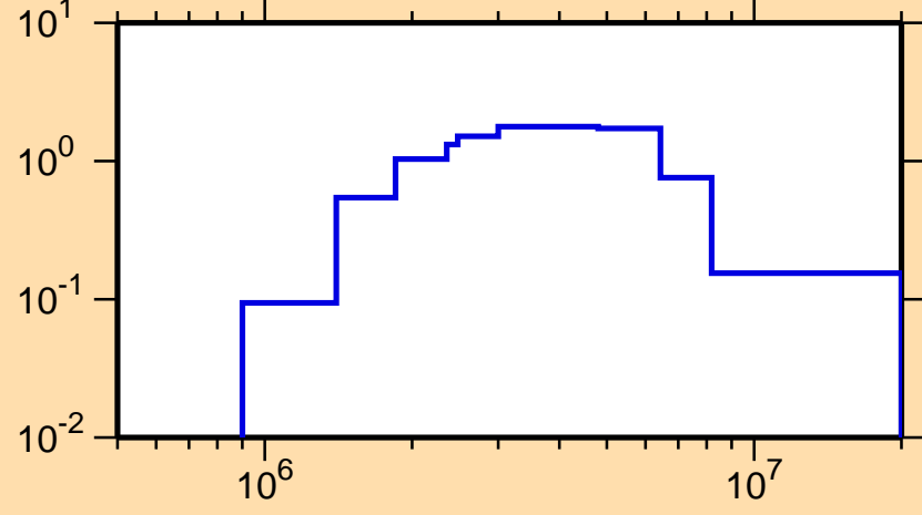
\sigma vs. E for ^{149}\text{La}(n,n\text{cont.})
