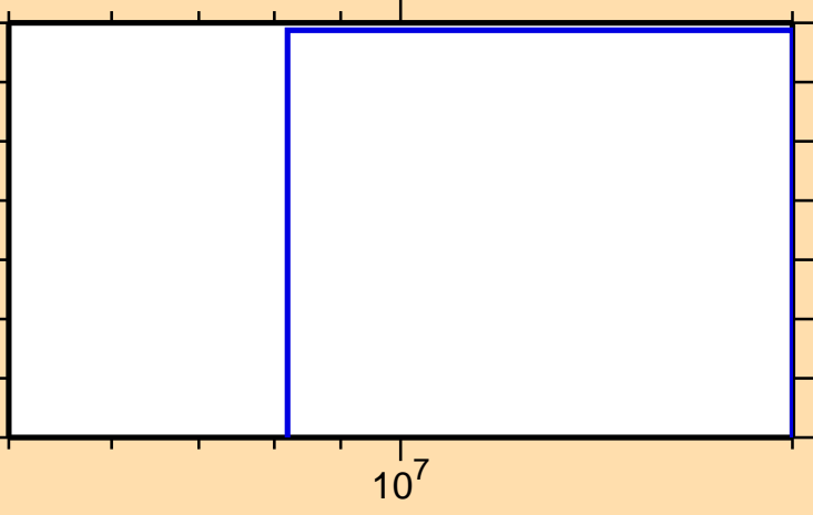
\sigma vs. E for ^{149}\text{La}(n,2n\alpha)
