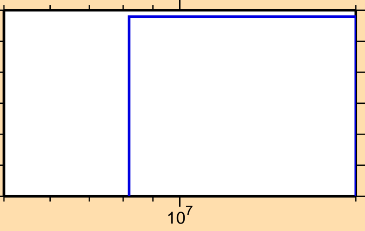
\sigma vs. E for ^{149}\text{La}(n,nt)
