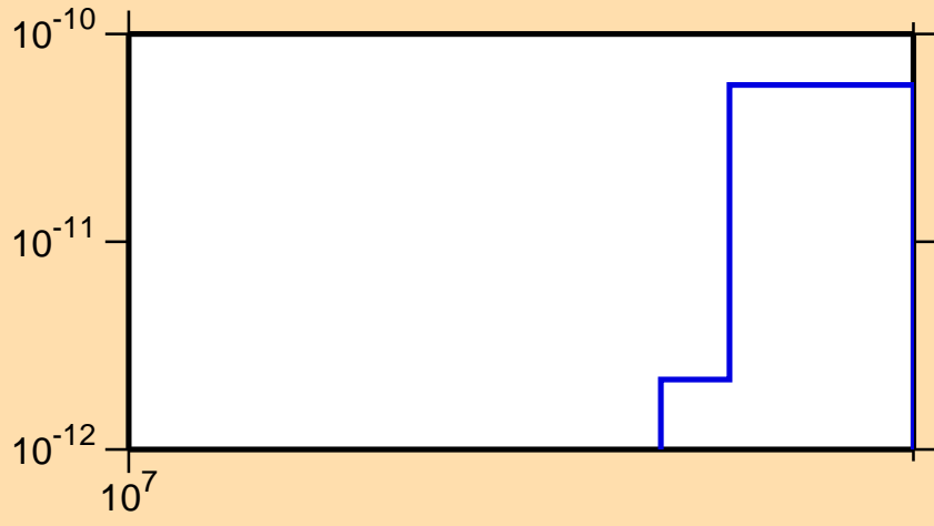
\sigma vs. E for ^{253}\text{Lw}(\text{mt 34})
