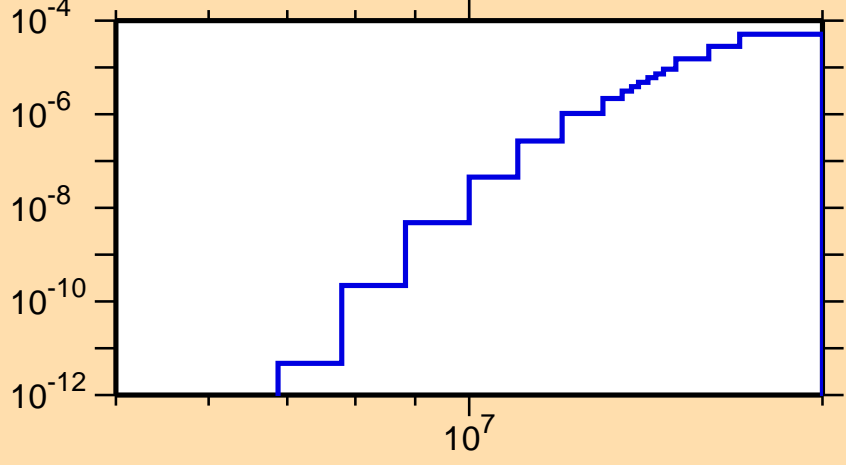
\sigma vs. E for ^{253}\text{Lw}(mt117)
