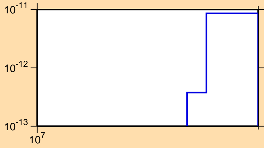
\sigma vs. E for ^{253}\text{Lw}(n,\text{pt})
