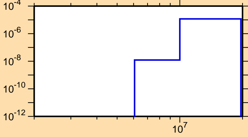
\sigma vs. E for ^{253}\text{Lw}(\text{mt } 45)
