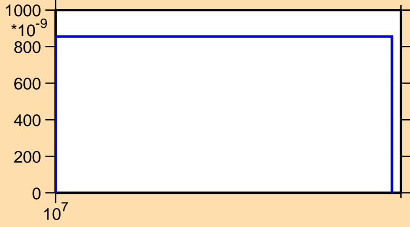
\sigma vs. E for ^{253}\text{Lw}(n,2np)
