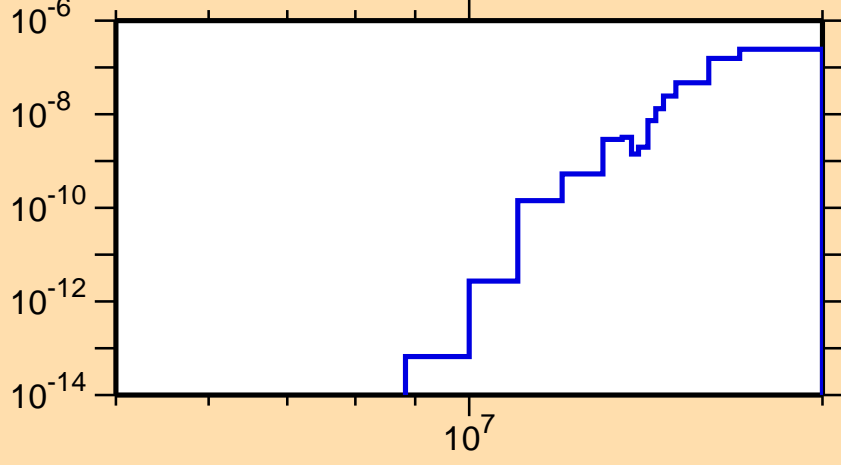
\sigma vs. E for ^{256}\text{Lw}(\text{mt } 45)
