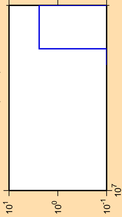
\Delta\sigma/\sigma vs. E for ^{256}\text{Lw}(mt\ 42)
