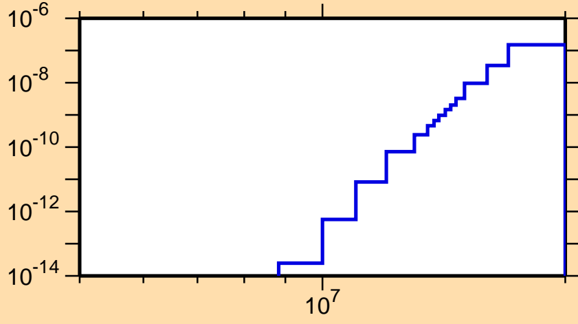
\sigma vs. E for ^{256}\text{Lw}(n,\text{He3})
