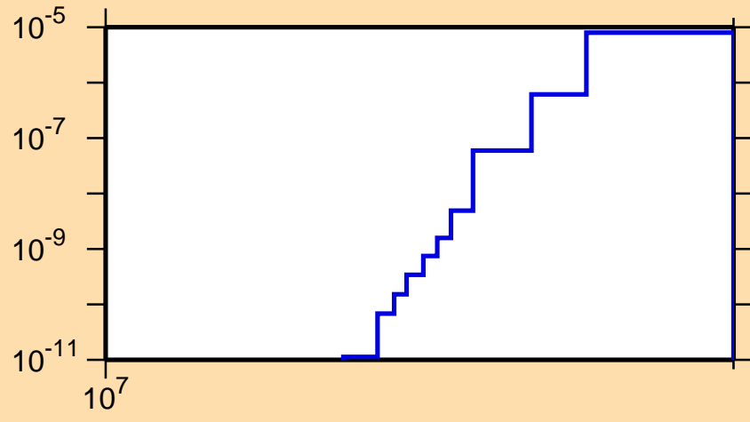
\sigma vs. E for ^{256}\text{Lw}(n,nt)
