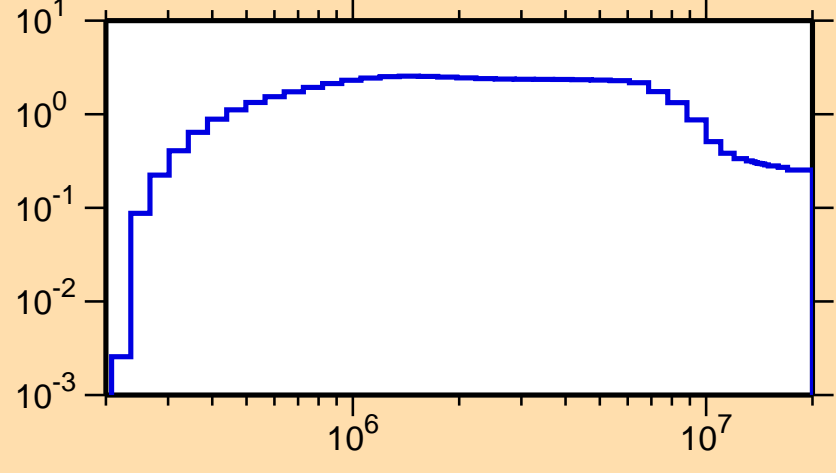
\sigma vs. E for ^{256}\text{Lw}(n,ncont.)
