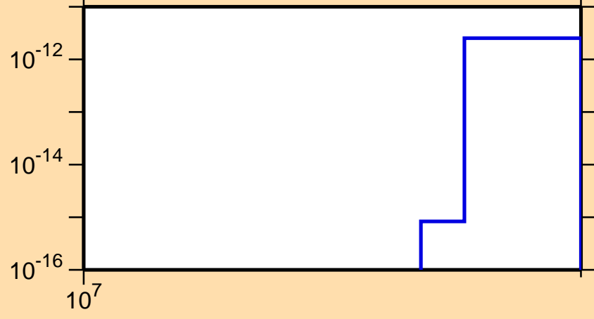
\sigma vs. E for ^{256}\text{Lw}(mt\ 42)
