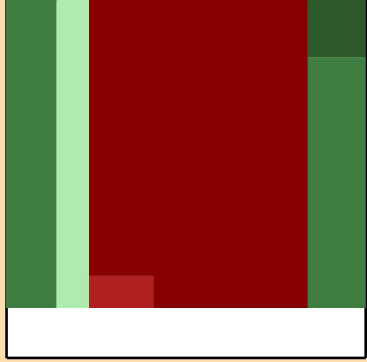
\Delta\sigma/\sigma vs. E for ^{256}\text{Lw}(n,\text{tot.})
