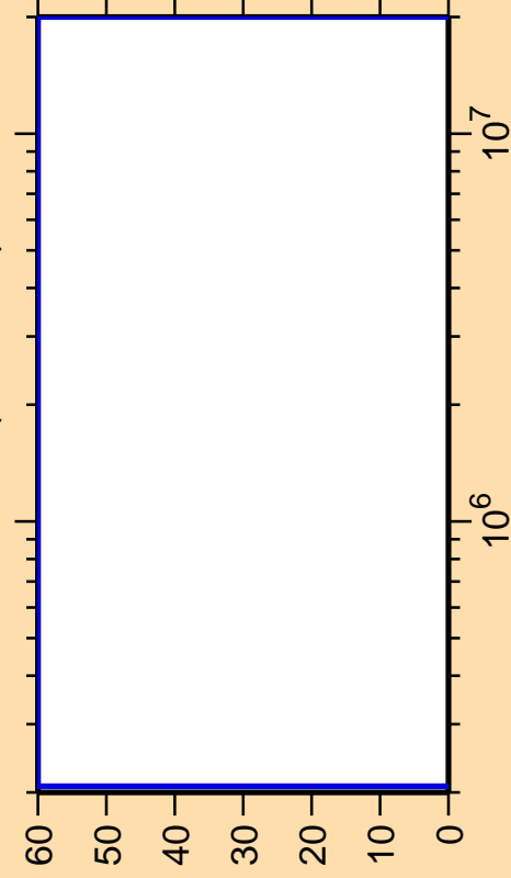
\Delta\sigma/\sigma vs. E for ^{256}\text{Lw}(n,ncont.)
