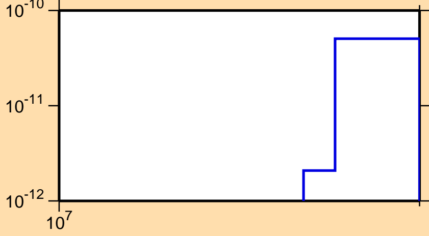
\sigma vs. E for ^{256}\text{Lw}(mt\ 34)
