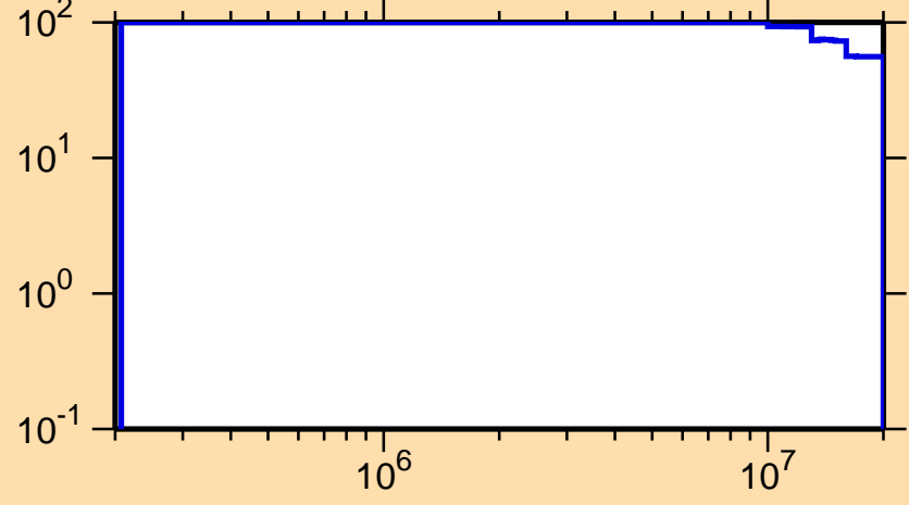
\Delta\sigma/\sigma vs. E for ^{256}\text{Lw}(n,f)
