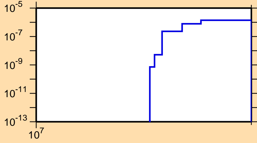
\sigma vs. E for ^{256}\text{Lw}(n,3n\alpha)
