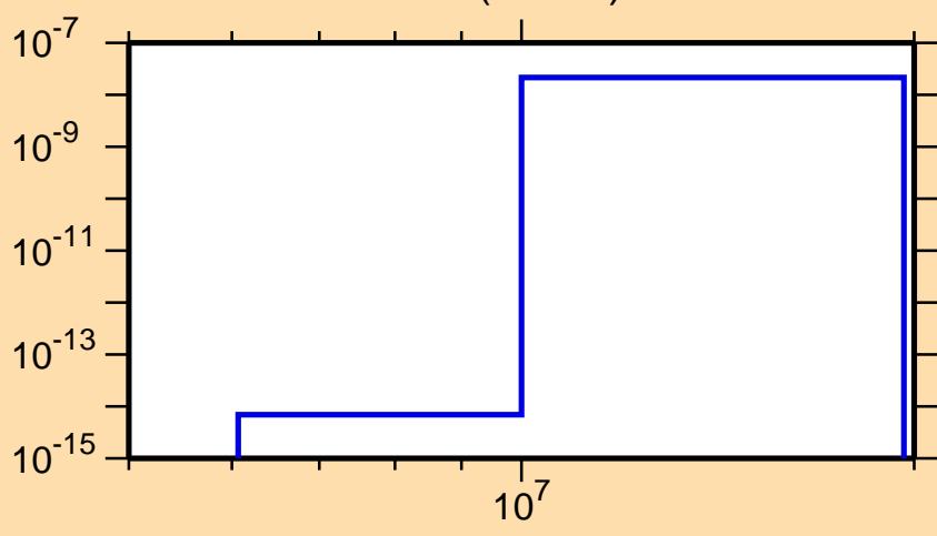
\sigma vs. E for ^{256}\text{Lw}(\text{mt } 45)
