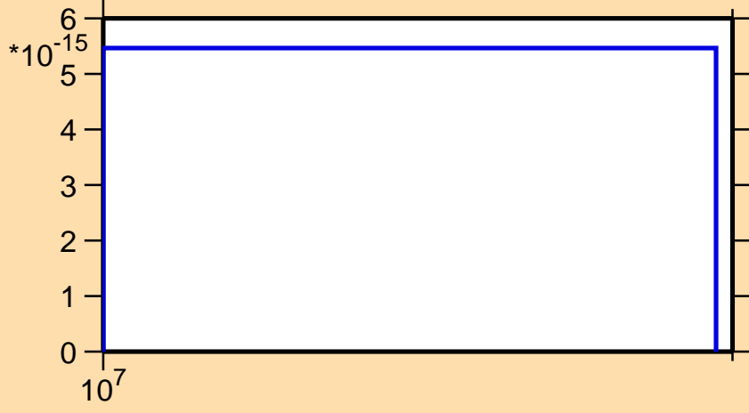
\sigma vs. E for ^{256}\text{Lw}(n,\text{pt})
