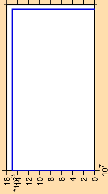
\Delta\sigma/\sigma vs. E for ^{256}\text{Lw}(n,\text{pd})
