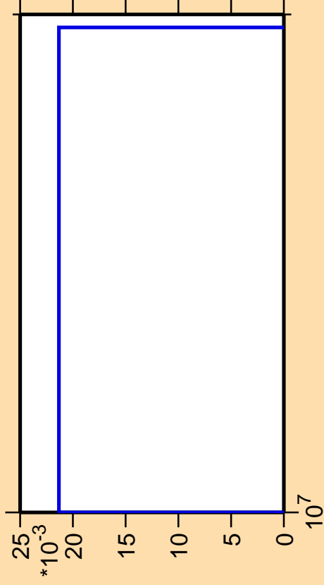
\Delta\sigma/\sigma vs. E for ^{256}\text{Lw}(mt\ 11)
