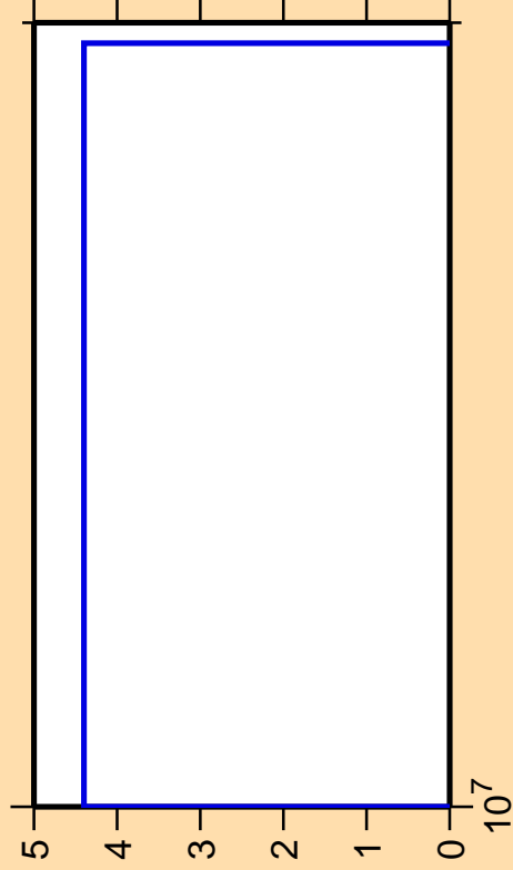
\Delta\sigma/\sigma vs. E for ^{256}\text{Lw}(\text{mt } 34)
