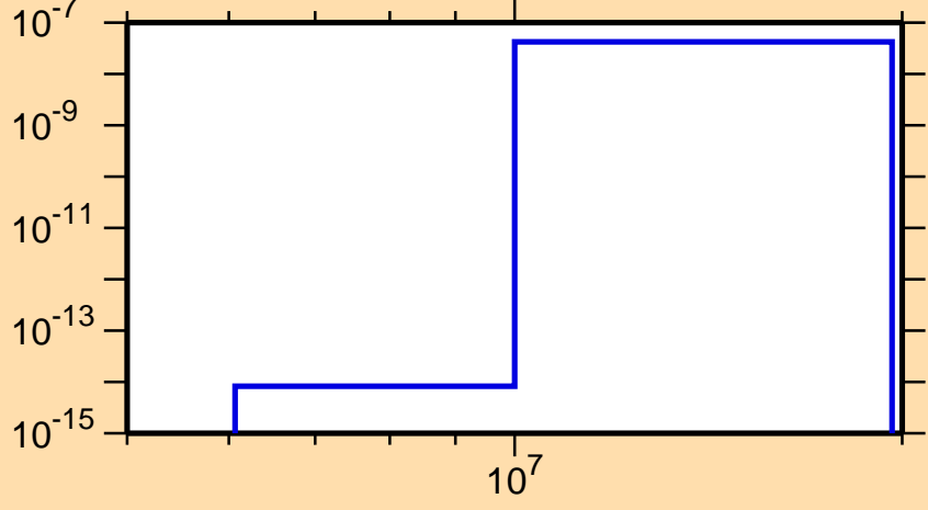
\sigma vs. E for ^{256}\text{Lw}(mt117)
