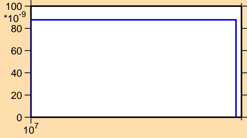
\sigma vs. E for ^{256}\text{Lw}(n,3n\alpha)
