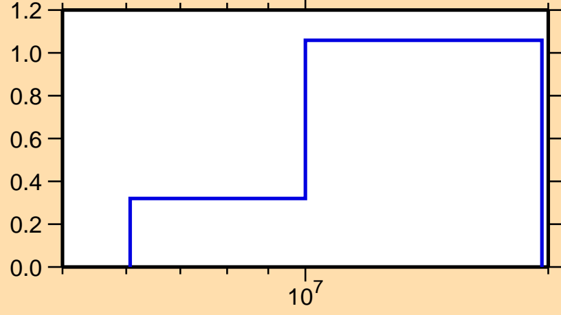
\sigma vs. E for ^{256}\text{Lw}(n,2n)
