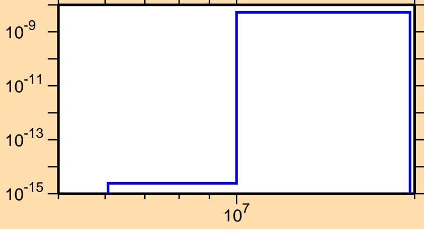
\sigma vs. E for ^{256}\text{Lw}(n,\text{He3})
