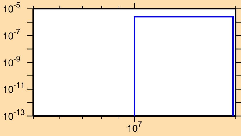
\sigma vs. E for ^{256}\text{Lw}(n,2np)
