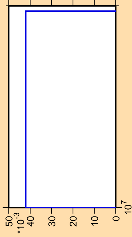
\Delta\sigma/\sigma vs. E for ^{256}\text{Lw}(n,\text{pt})
