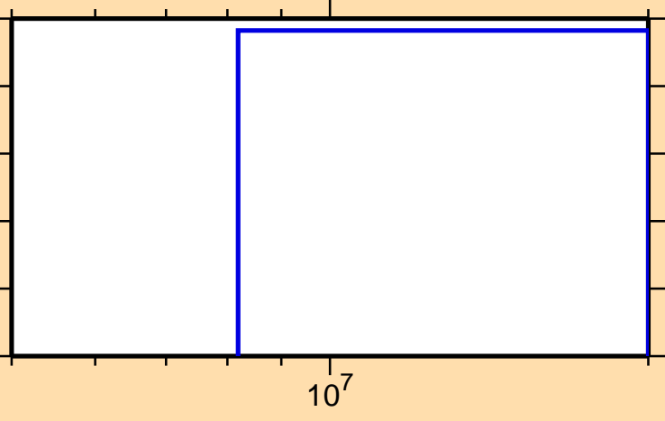
\sigma vs. E for ^{256}\text{Lw}(n,nt)
