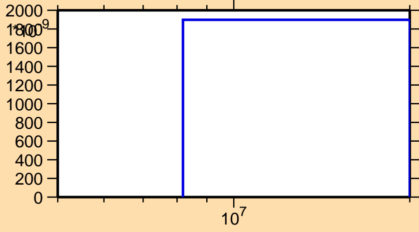
\sigma vs. E for ^{256}\text{Lw}(n,nd)
