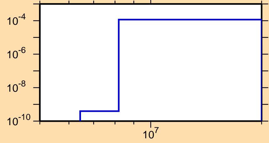
\sigma vs. E for ^{256}\text{Lw}(n,2n\alpha)
