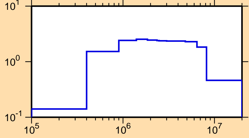
\sigma vs. E for ^{256}\text{Lw}(n,ncont.)
