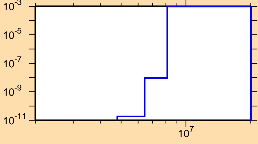
\sigma vs. E for ^{256}\text{Lw}(n,d)
