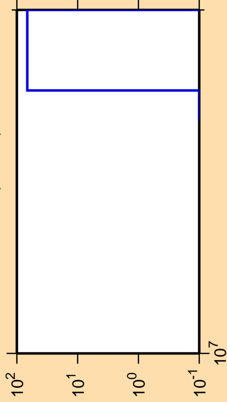
\Delta\sigma/\sigma vs. E for ^{257}\text{Lw}(\text{mt 11})
