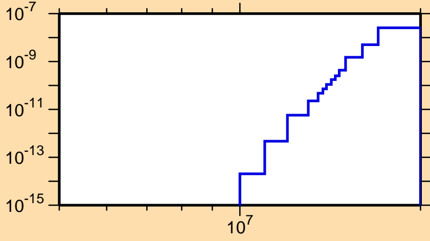
\sigma vs. E for ^{257}\text{Lw}(n,\text{He3})
