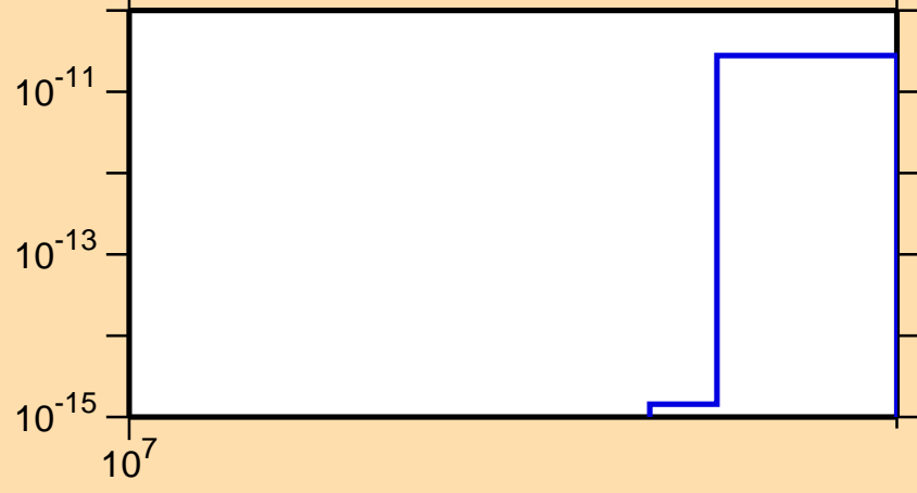
\sigma vs. E for ^{257}\text{Lw}(\text{mt 11})
