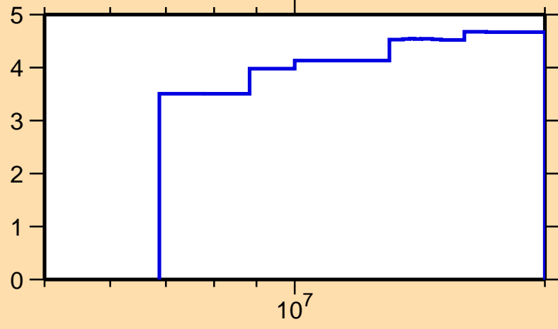
\Delta\sigma/\sigma vs. E for ^{257}\text{Lw}(n,\text{nonel.})
