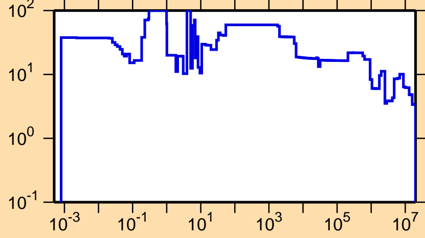
\Delta\sigma/\sigma vs. E for ^{257}\text{Lw}(n,\text{tot.})
