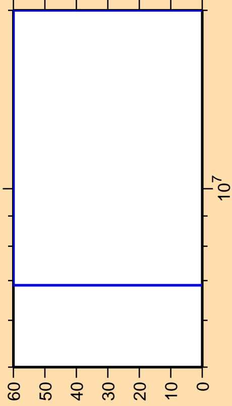
\Delta\sigma/\sigma vs. E for ^{257}\text{Lw}(n,\gamma)
