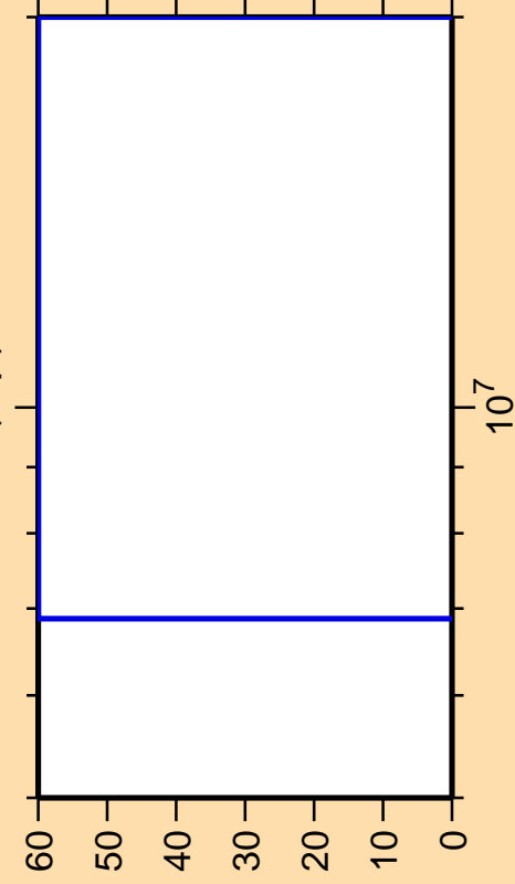
\Delta\sigma/\sigma vs. E for ^{257}\text{Lw}(n,p)
