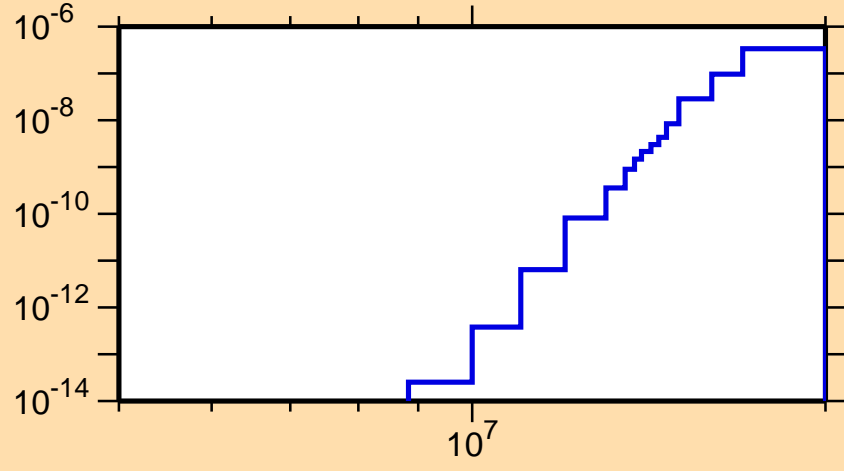
\sigma vs. E for ^{257}\text{Lw}(\text{mt117})
