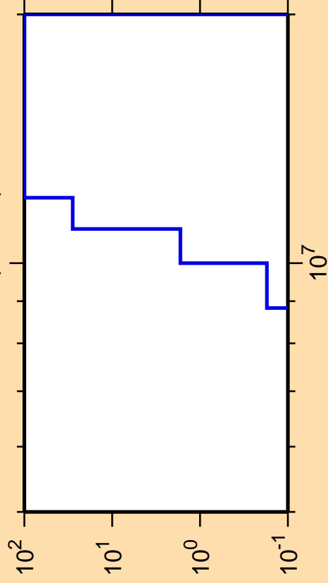
\Delta\sigma/\sigma vs. E for ^{257}\text{Lw}(\text{mt } 45)
