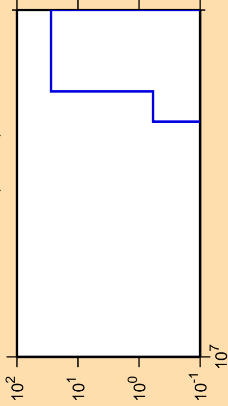
\Delta\sigma/\sigma vs. E for ^{257}\text{Lw}(\text{mt 34})
