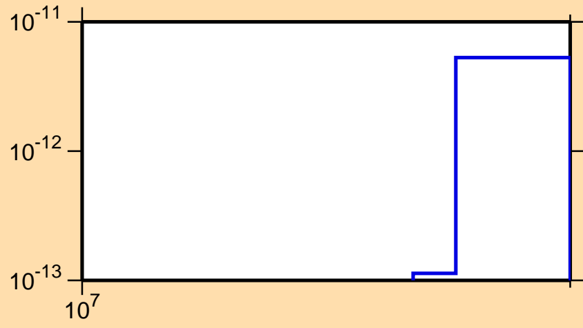
\sigma vs. E for ^{257}\text{Lw}(\text{mt 34})
