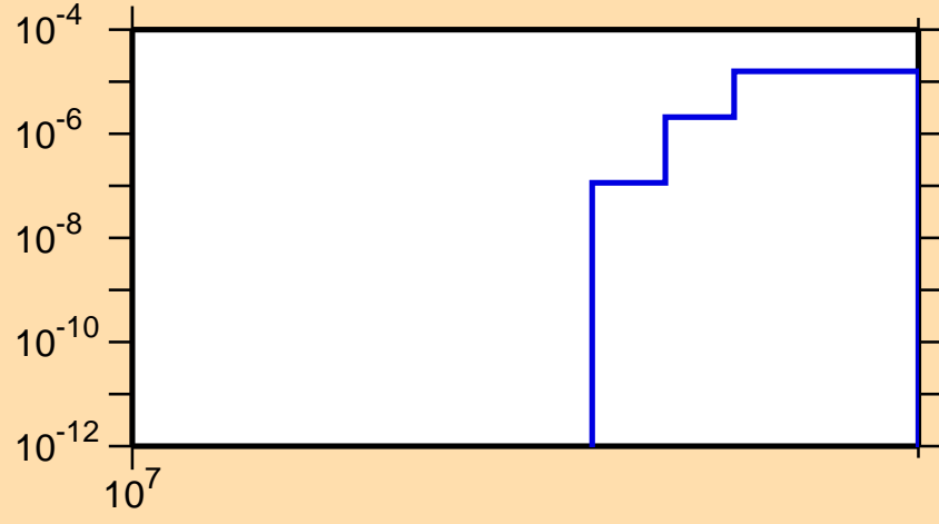
\sigma vs. E for ^{257}\text{Lw}(n,3n\alpha)
