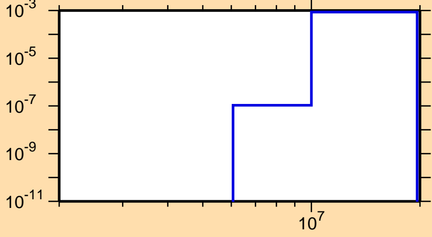
\sigma vs. E for ^{257}\text{Lw}(n,d)
