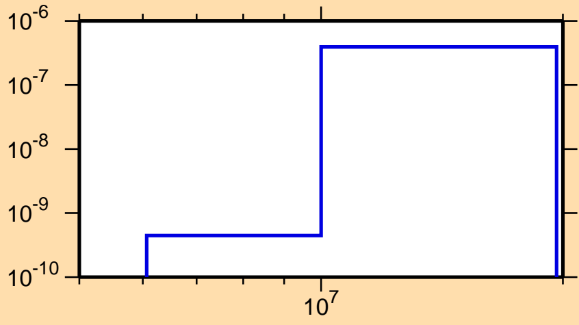
\sigma vs. E for ^{257}\text{Lw}(n,p\alpha)
