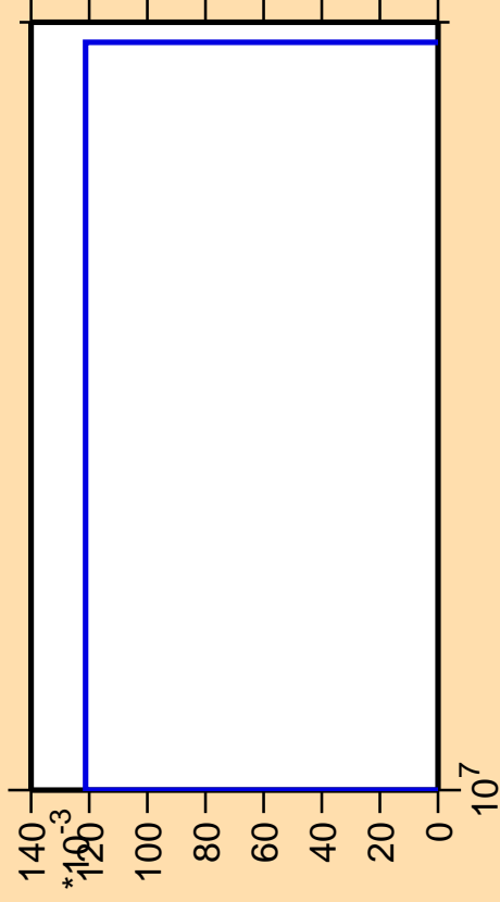
\Delta\sigma/\sigma vs. E for ^{257}\text{Lw}(\text{mt } 42)
