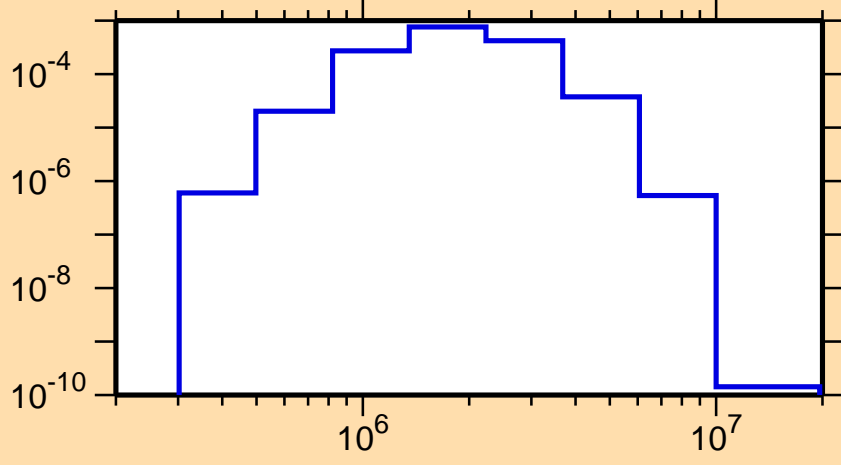
\sigma vs. E for ^{257}\text{Lw}(n,n_4)
