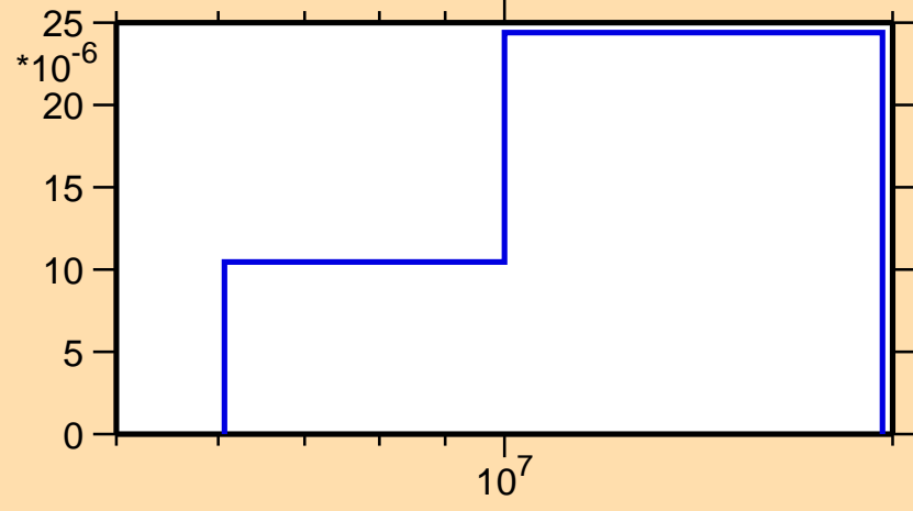
\sigma vs. E for ^{257}\text{Lw}(n,2n\alpha)
