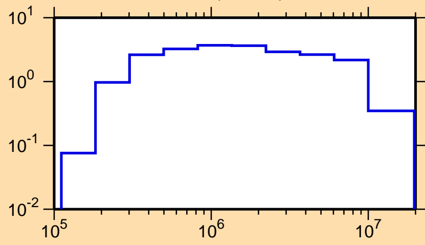
\sigma vs. E for ^{257}\text{Lw}(n,\text{inel.})
