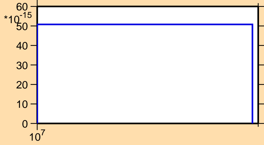
\sigma vs. E for ^{257}\text{Lw}(\text{mt 34})
