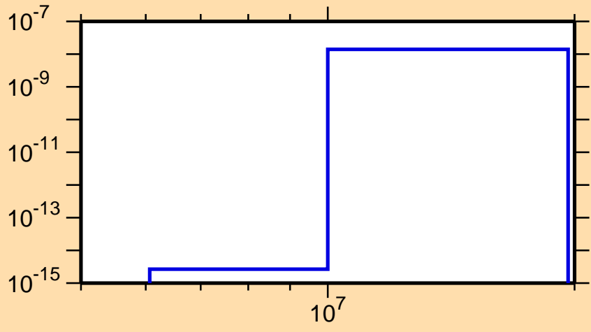
\sigma vs. E for ^{257}\text{Lw}(\text{mt117})
