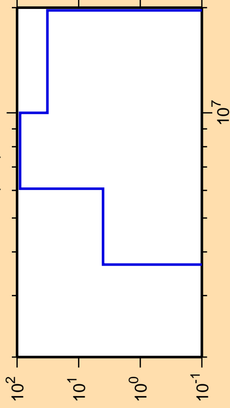
\Delta\sigma/\sigma vs. E for ^{257}\text{Lw}(n,d)
