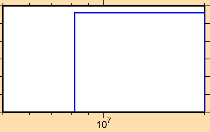
\sigma vs. E for ^{257}\text{Lw}(n,nt)
