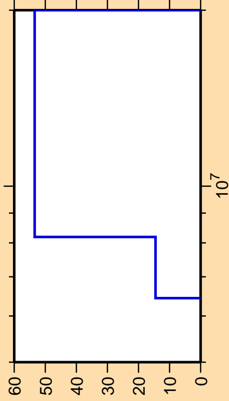
\Delta\sigma/\sigma vs. E for ^{257}\text{Lw}(n,t)
