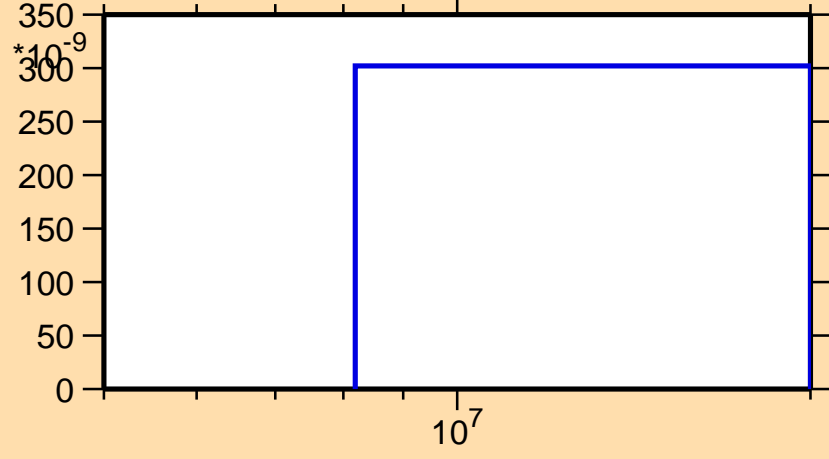
\sigma vs. E for ^{257}\text{Lw}(n,nd)
