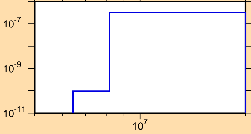
\sigma vs. E for ^{257}\text{Lw}(n,p\alpha)
