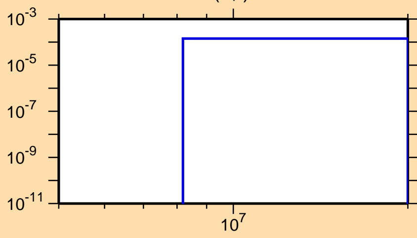
\sigma vs. E for ^{257}\text{Lw}(n,t)
