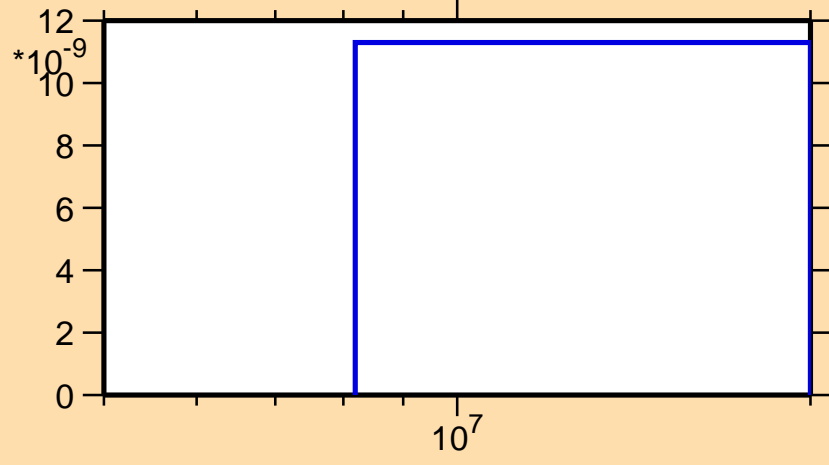
\sigma vs. E for ^{257}\text{Lw(mt117)}
