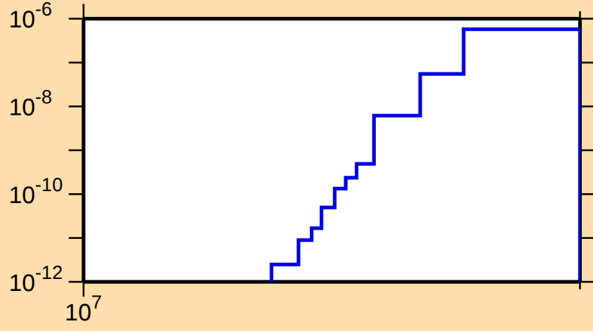
\sigma vs. E for ^{263}\text{Lw}(n,nd)
