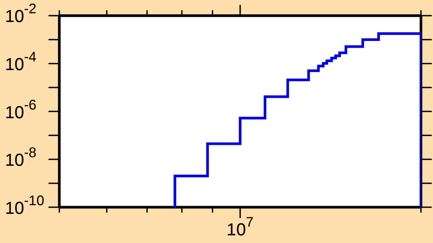
\sigma vs. E for ^{263}\text{Lw}(n,d)
