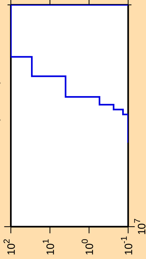
\Delta\sigma/\sigma vs. E for ^{263}\text{Lw}(n,\text{He3})
