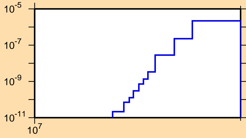
\sigma vs. E for ^{264}\text{Lw}(n,nt)
