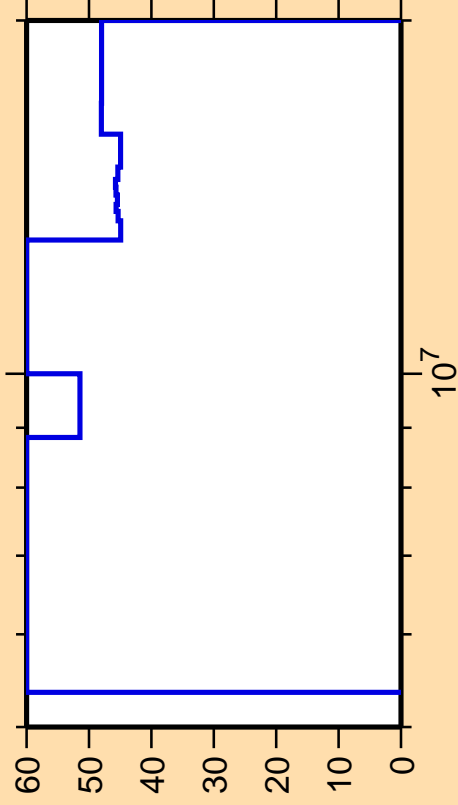
\Delta\sigma/\sigma vs. E for ^{264}\text{Lw}(n,\gamma)
