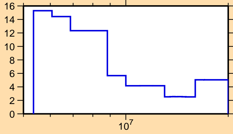
\Delta\sigma/\sigma vs. E for ^{264}\text{Lw}(n,\text{tot.})
