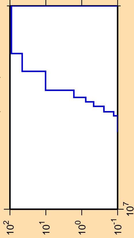
\Delta\sigma/\sigma vs. E for ^{264}\text{Lw}(n,\text{He3})
