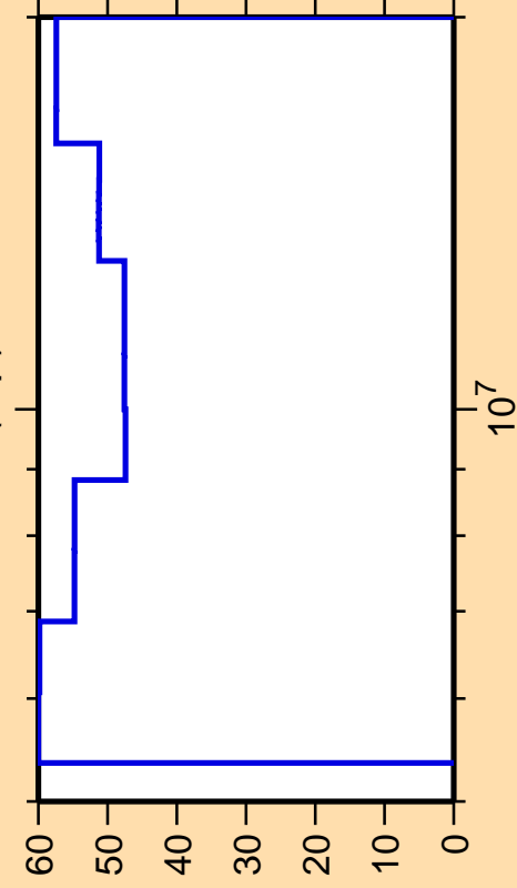
\Delta\sigma/\sigma vs. E for ^{264}\text{Lw}(n,p)
