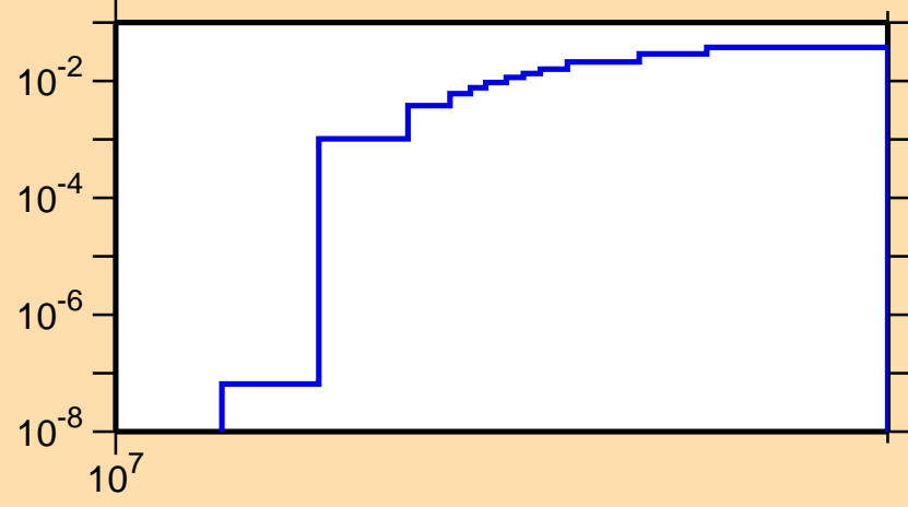
\sigma vs. E for ^{264}\text{Lw}(n,3n)
