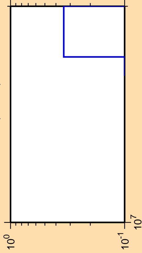
\Delta\sigma/\sigma vs. E for ^{264}\text{Lw(mt 11)}
