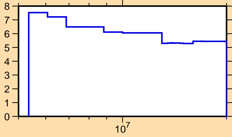
\Delta\sigma/\sigma vs. E for ^{264}\text{Lw}(n,\text{nonel.})
