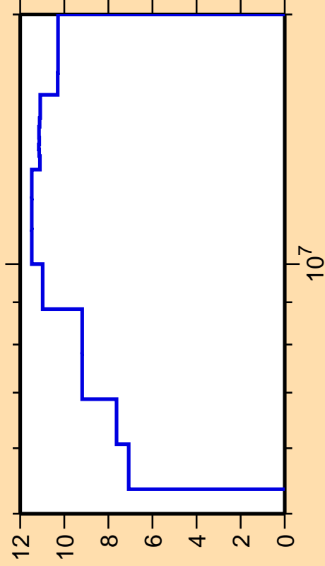
\Delta\sigma/\sigma vs. E for ^{264}\text{Lw}(n,f)
