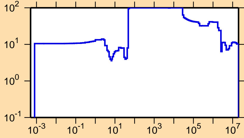
\Delta\sigma/\sigma vs. E for ^{264}\text{Lw}(n,f)
