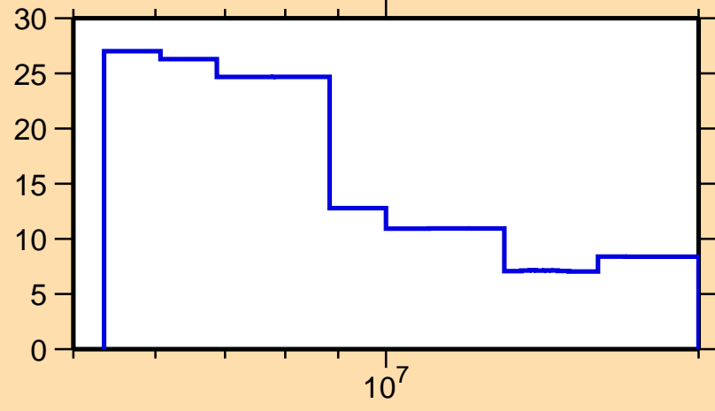
\Delta\sigma/\sigma vs. E for ^{264}\text{Lw}(n,\text{el.})
