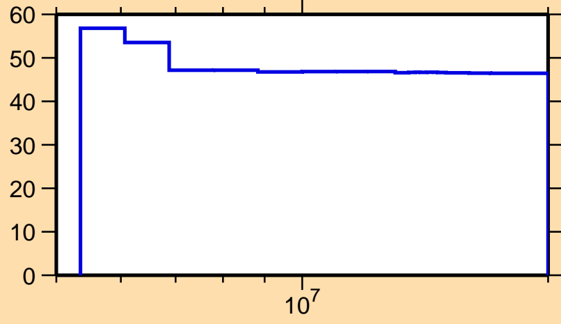
\Delta\sigma/\sigma vs. E for ^{264}\text{Lw}(n,\text{inel.})
