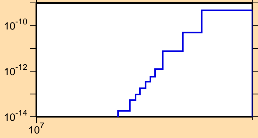
\sigma vs. E for ^{264}\text{Lw}(n,\text{He3})
