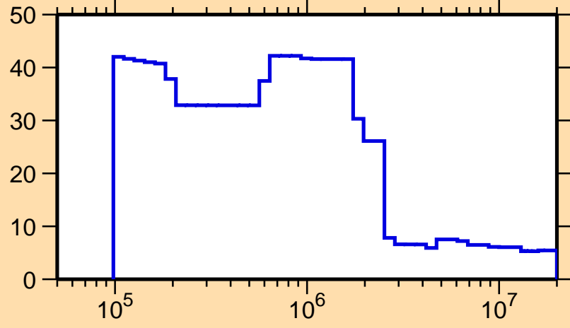
\Delta\sigma/\sigma vs. E for ^{264}\text{Lw}(n,\text{nonel.})
