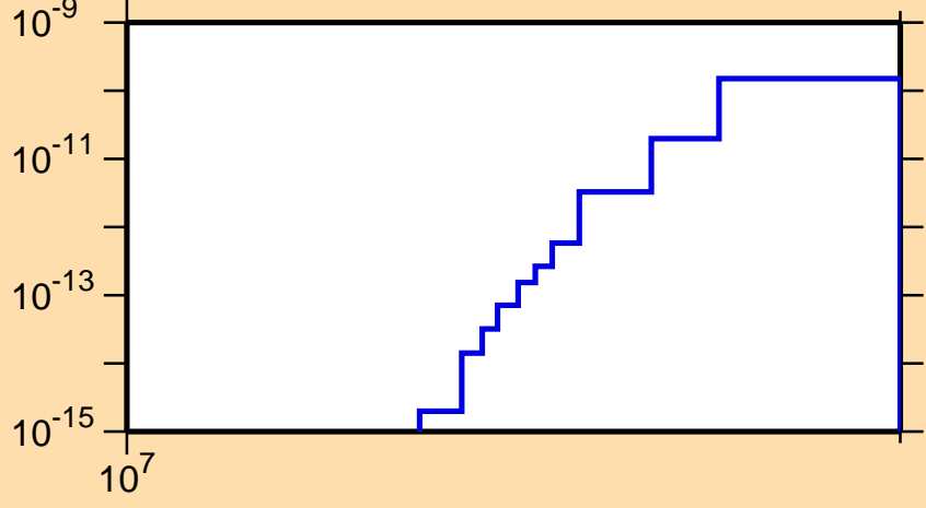
\sigma vs. E for ^{264}\text{Lw}(n,3n\alpha)
