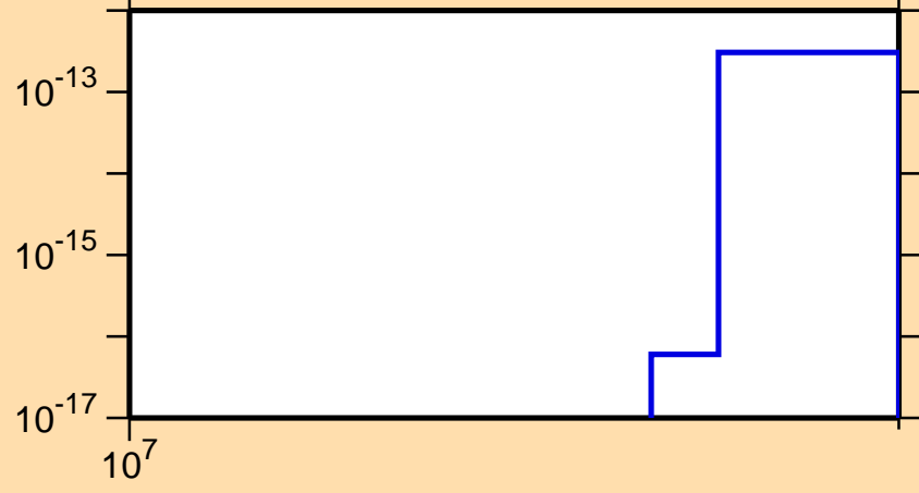
\sigma vs. E for ^{264}\text{Lw(mt 11)}
