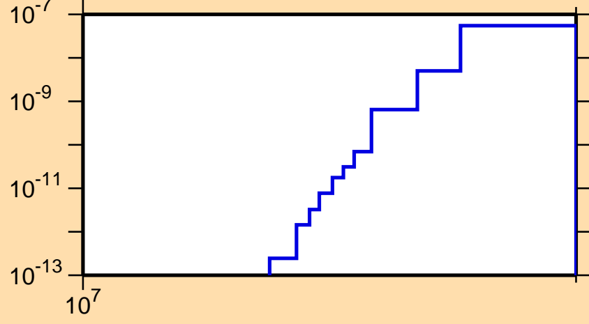
\sigma vs. E for ^{264}\text{Lw}(n,2np)
