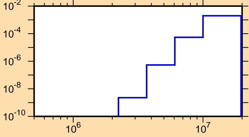
\sigma vs. E for ^{264}\text{Lw}(n,p)
