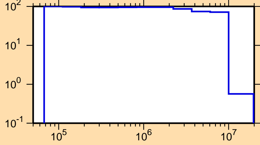
\Delta\sigma/\sigma vs. E for ^{264}\text{Lw}(n,n_1)
