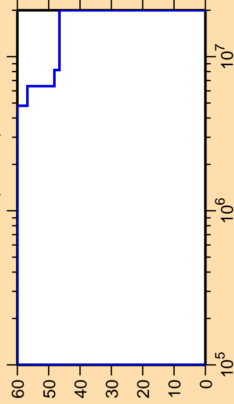
\Delta\sigma/\sigma vs. E for ^{264}\text{Lw}(n,\text{inel.})
