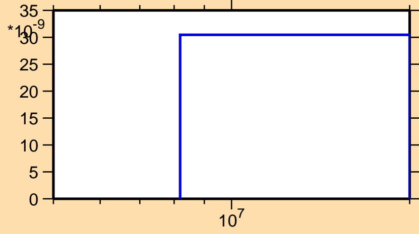
\sigma vs. E for ^{264}\text{Lw}(n,nt)
