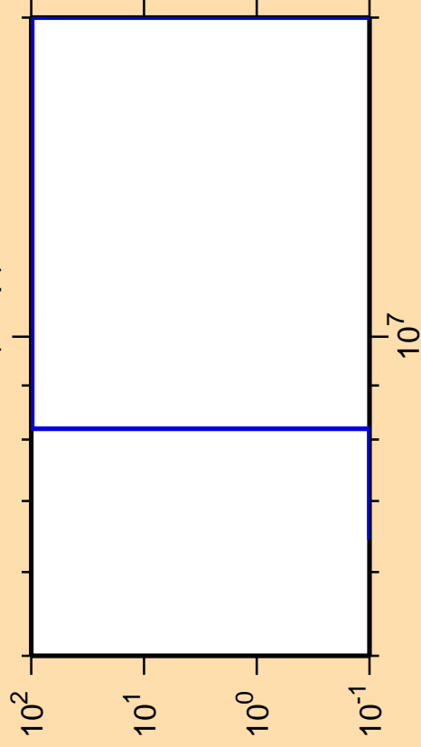
\Delta\sigma/\sigma vs. E for ^{264}\text{Lw}(n,np)
