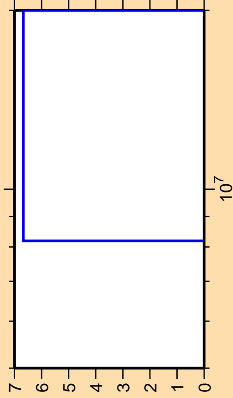
\Delta\sigma/\sigma vs. E for ^{264}\text{Lw}(n,\text{He3})
