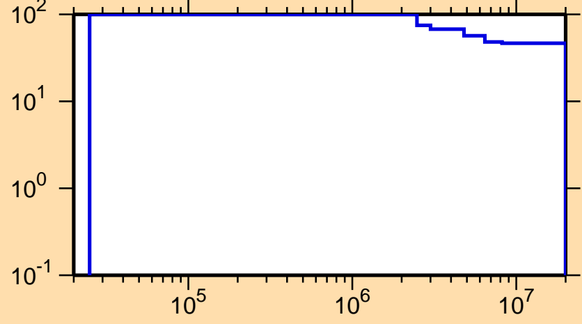
\Delta\sigma/\sigma vs. E for ^{264}\text{Lw}(n,\text{inel.})
