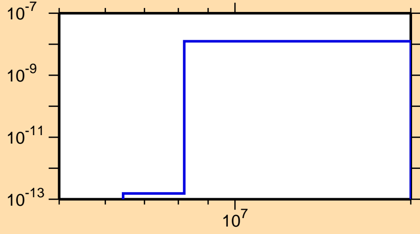
\sigma vs. E for ^{264}\text{Lw}(n,2n\alpha)
