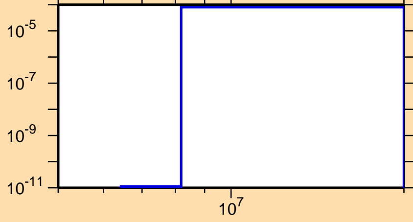
\sigma vs. E for ^{264}\text{Lw}(n,t)
