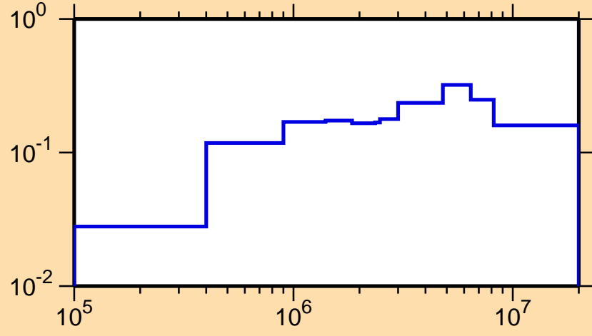
\sigma vs. E for ^{264}\text{Lw}(n,\text{inel.})
