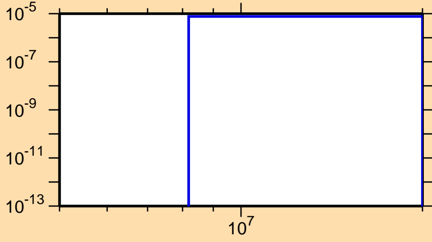
\sigma vs. E for ^{264}\text{Lw}(n,np)
