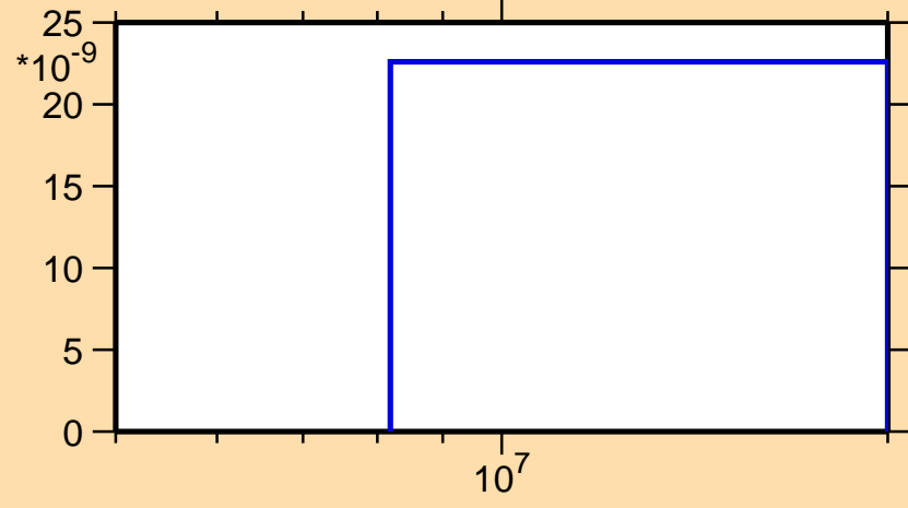
\sigma vs. E for ^{264}\text{Lw}(n,nd)
