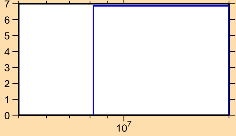
\Delta\sigma/\sigma vs. E for ^{154}\text{Lu}(n,\text{nonel.})
