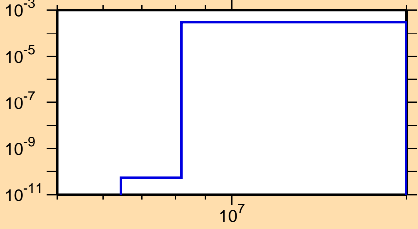
\sigma vs. E for ^{154}\text{Lu}(n,\text{pd})
