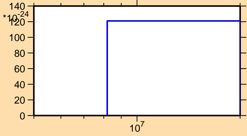
\sigma vs. E for ^{154}\text{Lu}(\text{mt 11})
