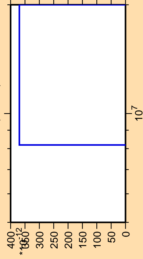
\Delta\sigma/\sigma vs. E for ^{154}\text{Lu}(\text{mt 11})
