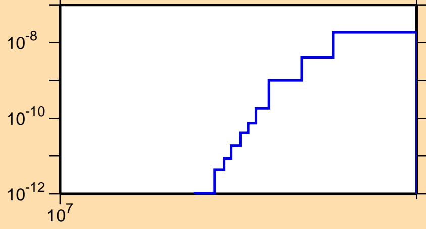
\sigma vs. E for ^{154}\text{Lu}(n,2n\alpha)
