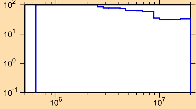
\Delta\sigma/\sigma vs. E for ^{154}\text{Lu}(n,n\text{cont.})
