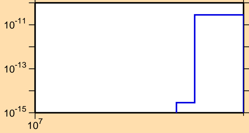
\sigma vs. E for ^{154}\text{Lu}(n,nt)
