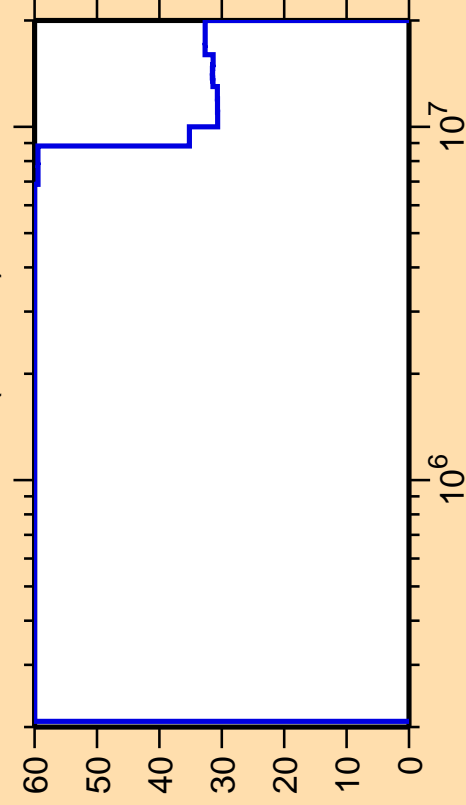
\Delta\sigma/\sigma vs. E for ^{154}\text{Lu}(n,\text{inel.})
