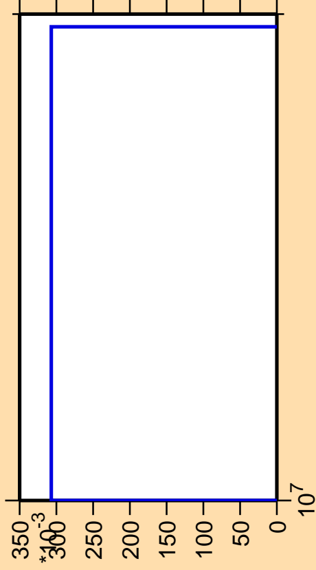
\Delta\sigma/\sigma vs. E for ^{154}\text{Lu}(n,nt)
