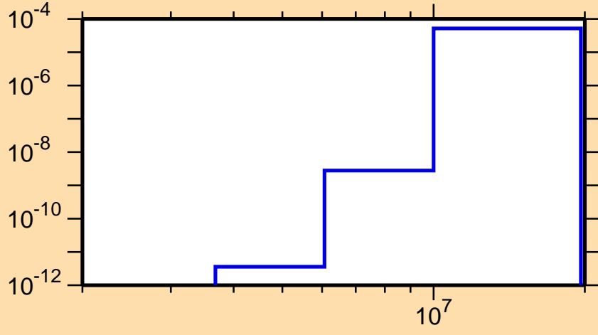
\sigma vs. E for ^{154}\text{Lu}(\text{mt } 45)
