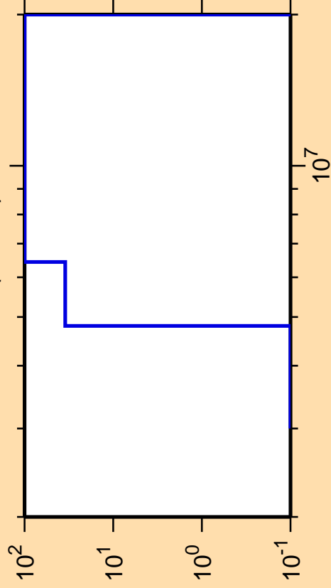
\Delta\sigma/\sigma vs. E for ^{154}\text{Lu} (mt 45)
