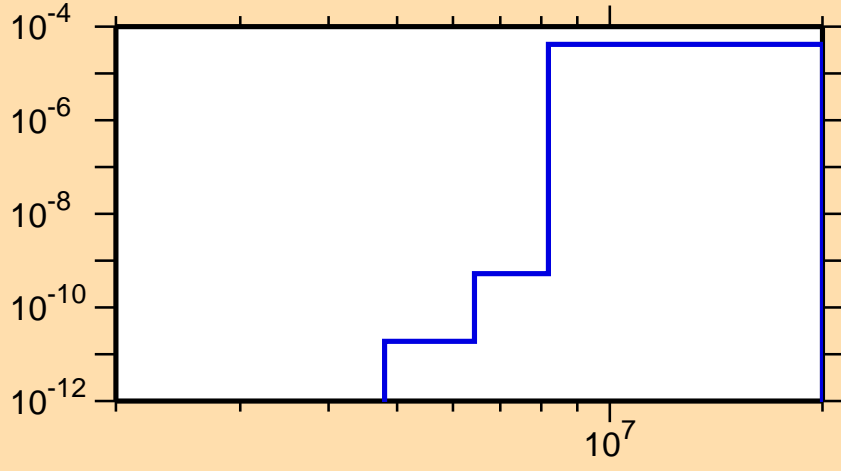
\sigma vs. E for ^{154}\text{Lu} (mt 45)
