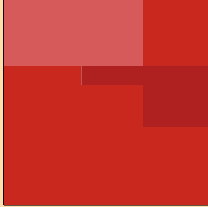
\Delta\sigma/\sigma vs. E for ^{157}\text{Lu}(n,2n)
