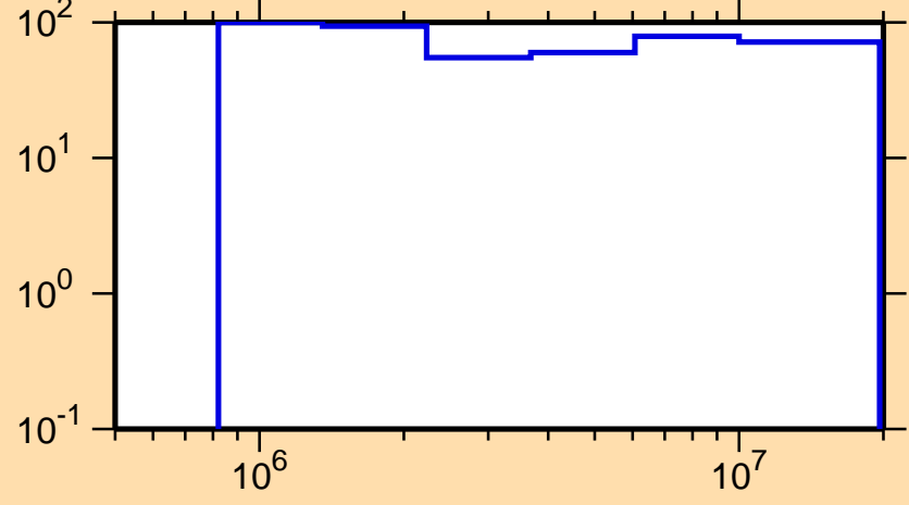
\Delta\sigma/\sigma vs. E for ^{157}\text{Lu}(n,ncont.)
