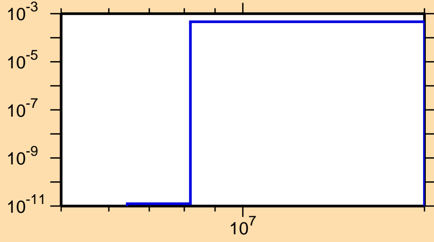
\sigma vs. E for ^{157}\text{Lu}(n,t)
