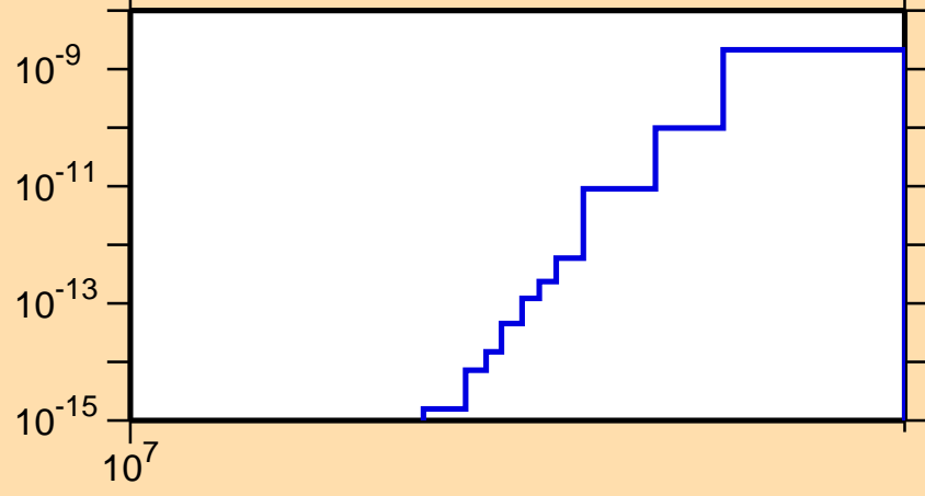
\sigma vs. E for ^{157}\text{Lu} (mt 34)
