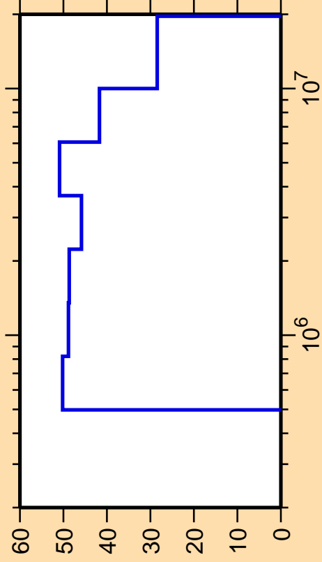
\Delta\sigma/\sigma vs. E for ^{157}\text{Lu}(n,n_3)
