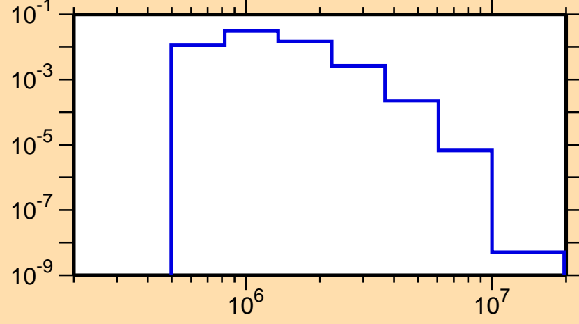
\sigma vs. E for ^{157}\text{Lu}(n,n_3)
