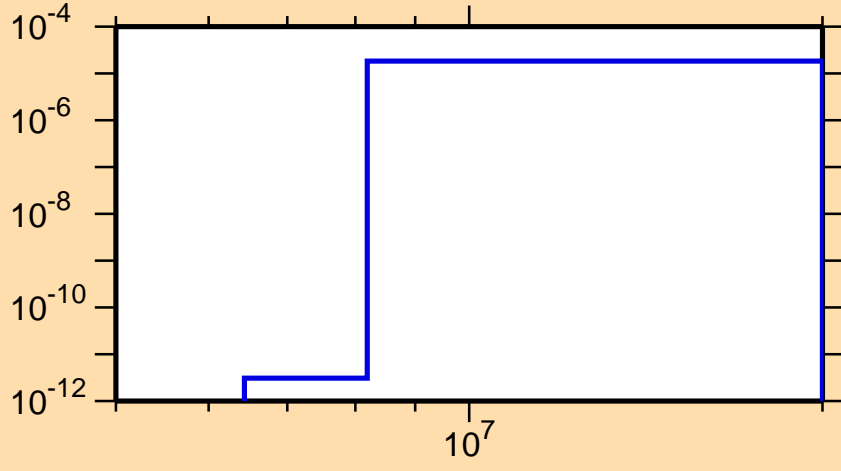
\sigma vs. E for ^{160}\text{Lu} (mt 45)
