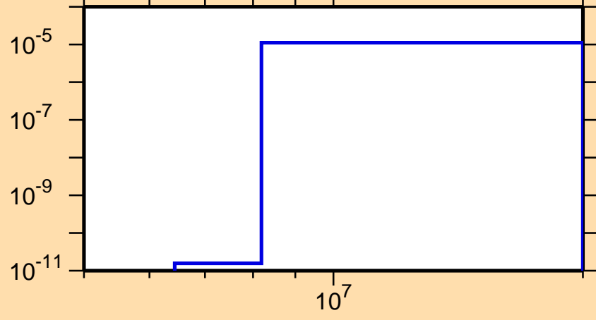
\sigma vs. E for ^{160}\text{Lu}(n,\text{He}3)
