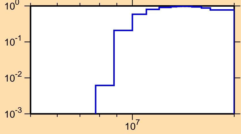
\sigma vs. E for ^{160}\text{Lu}(n,2n)
