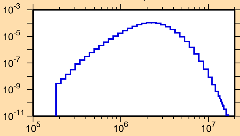
\sigma vs. E for ^{160}\text{Lu}(n,n_4)
