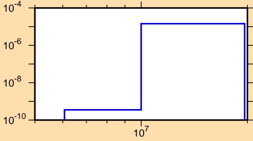
\sigma vs. E for ^{160}\text{Lu}(n,\text{He3})
