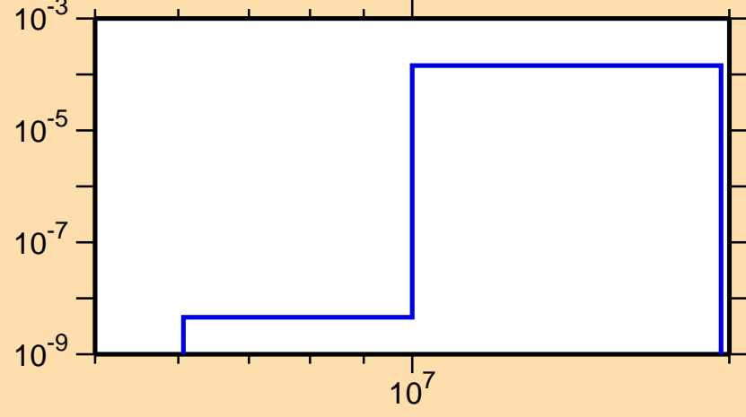
\sigma vs. E for ^{160}\text{Lu} (mt 45)
