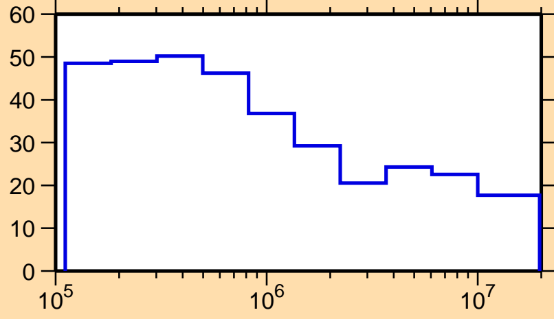
\Delta\sigma/\sigma vs. E for ^{161}\text{Lu}(n,nonel.)
