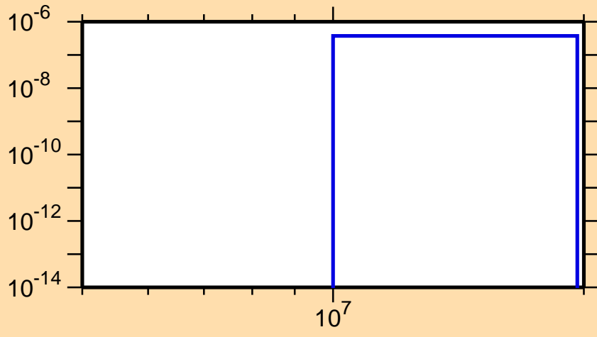
\sigma vs. E for ^{161}\text{Lu}(n,2n\alpha)
