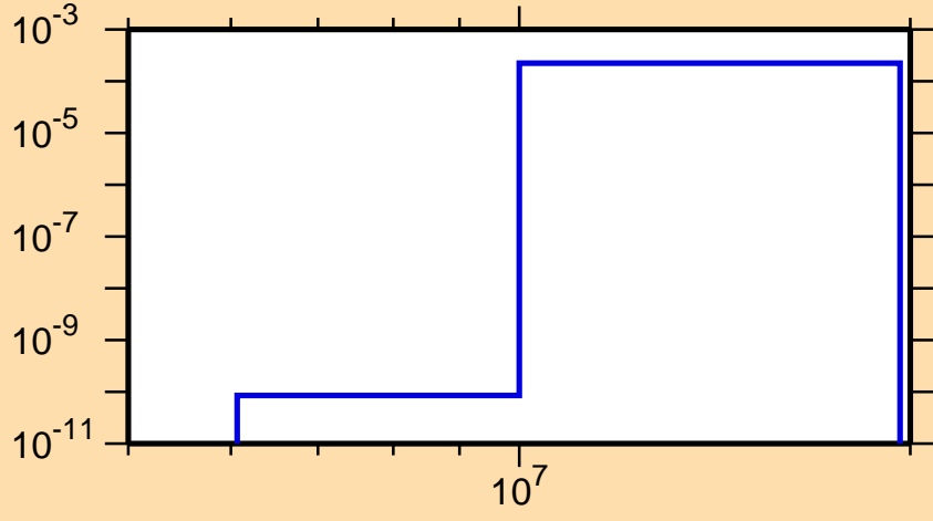
\sigma vs. E for ^{161}\text{Lu}(n,t)
