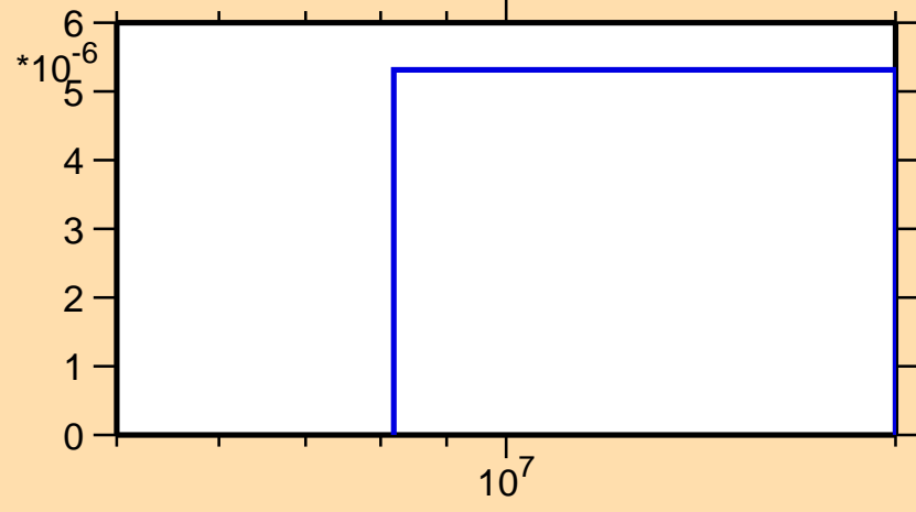
\sigma vs. E for ^{161}\text{Lu} (mt 45)
