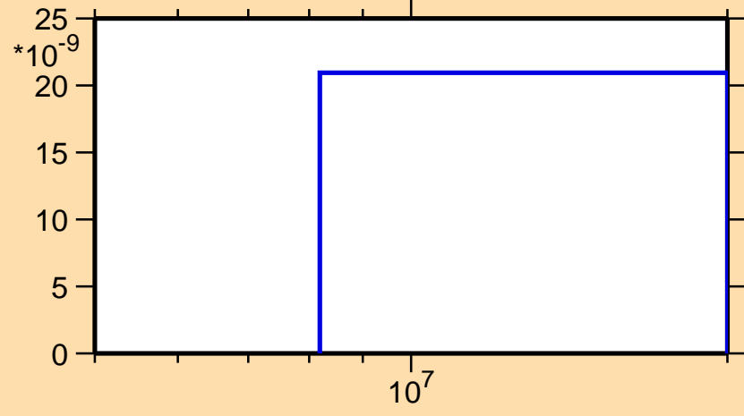
\sigma vs. E for ^{161}\text{Lu}(n,pd)
