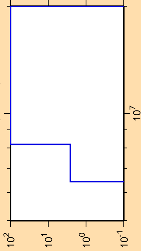
\Delta\sigma/\sigma vs. E for ^{161}\text{Lu}(n,\text{He}3)
