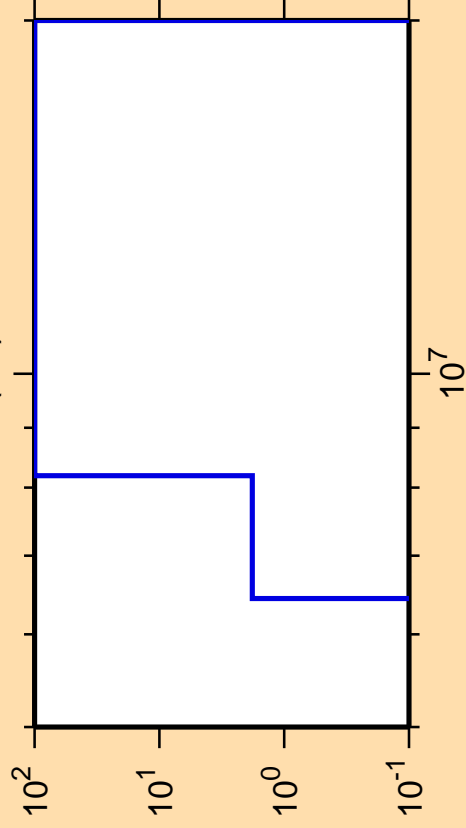
\Delta\sigma/\sigma vs. E for ^{161}\text{Lu}(n,t)
