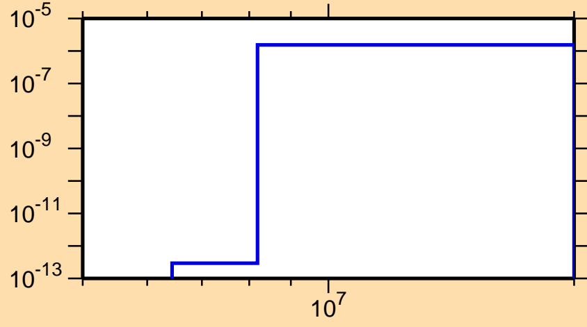
\sigma vs. E for ^{161}\text{Lu}(n,\text{He}3)
