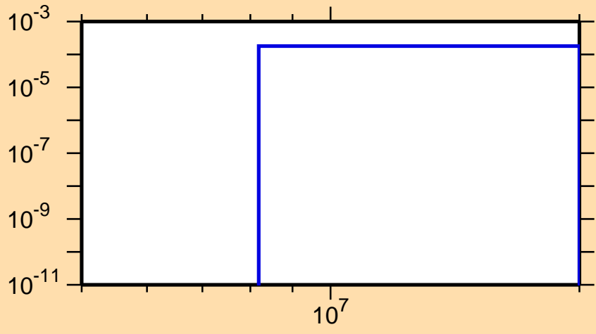
\sigma vs. E for ^{161}\text{Lu}(n,t)
