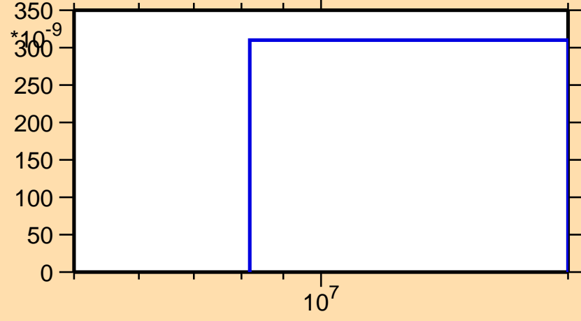
\sigma vs. E for ^{161}\text{Lu}(n,2n\alpha)
