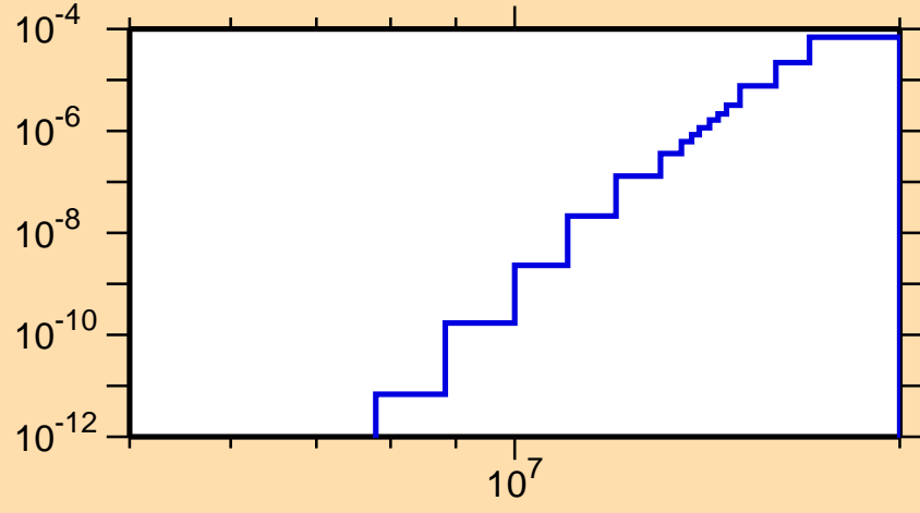
\sigma vs. E for ^{162}\text{Lu}(n,\text{He3})
