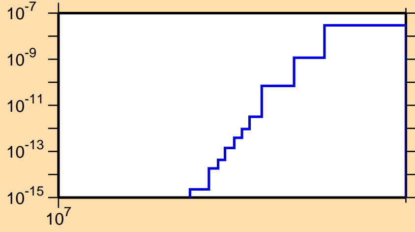
\sigma vs. E for ^{162}\text{Lu}(n,pt)
