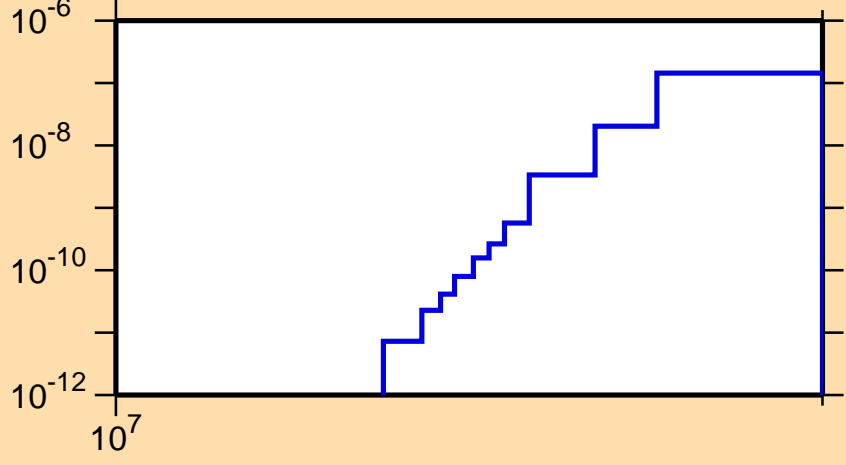
\sigma vs. E for ^{162}\text{Lu}(n,pd)
