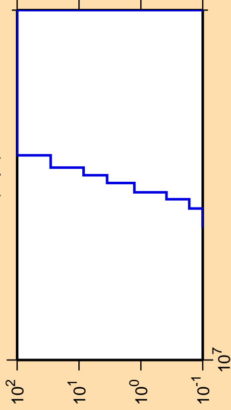
\Delta\sigma/\sigma vs. E for ^{162}\text{Lu}(n,pt)
