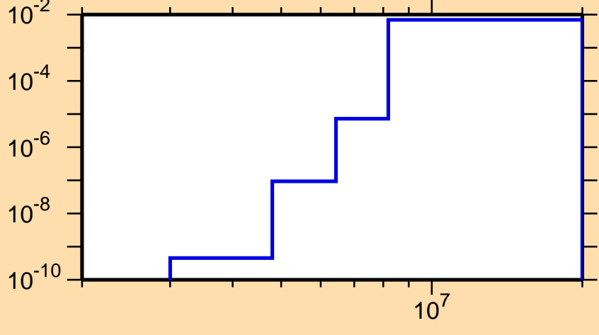
\sigma vs. E for ^{162}\text{Lu}(n,d)
