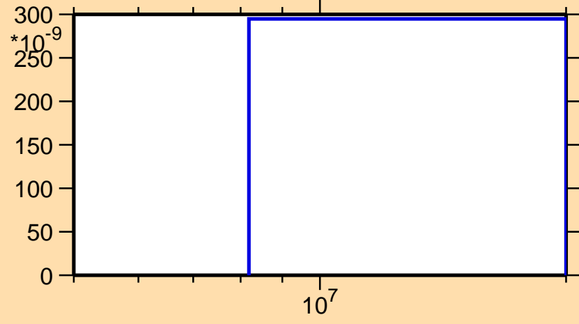
\sigma vs. E for ^{162}\text{Lu}(\text{mt } 45)
