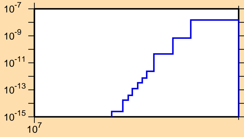
\sigma vs. E for ^{162}\text{Lu}(n,pt)
