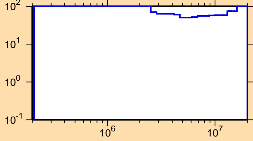
\Delta\sigma/\sigma vs. E for ^{162}\text{Lu}(n,n\text{cont.})
